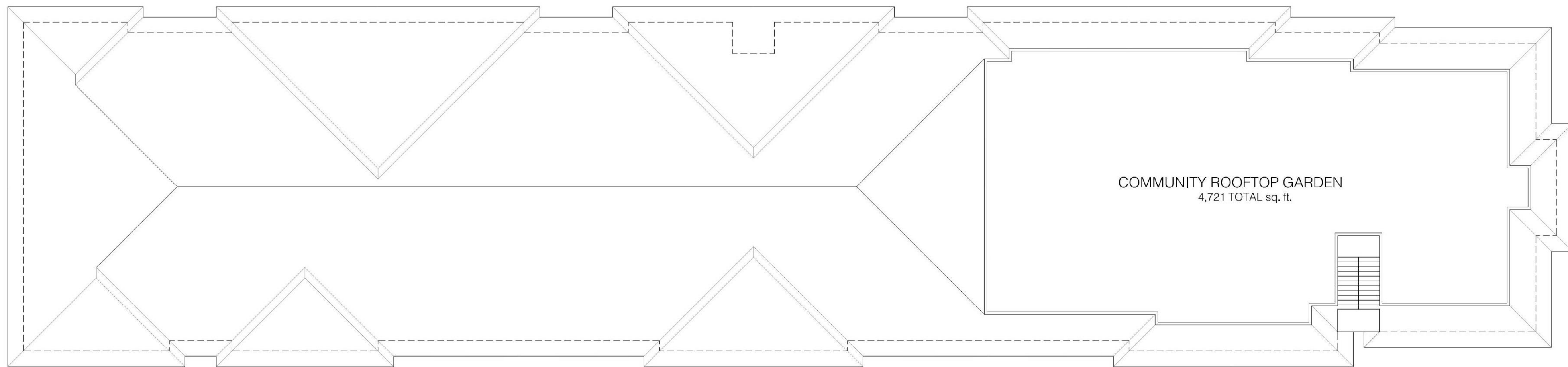
3 SOUTH BUILDING - THIRD FLOOR PLAN SCALE: 1" = 10'-0"
