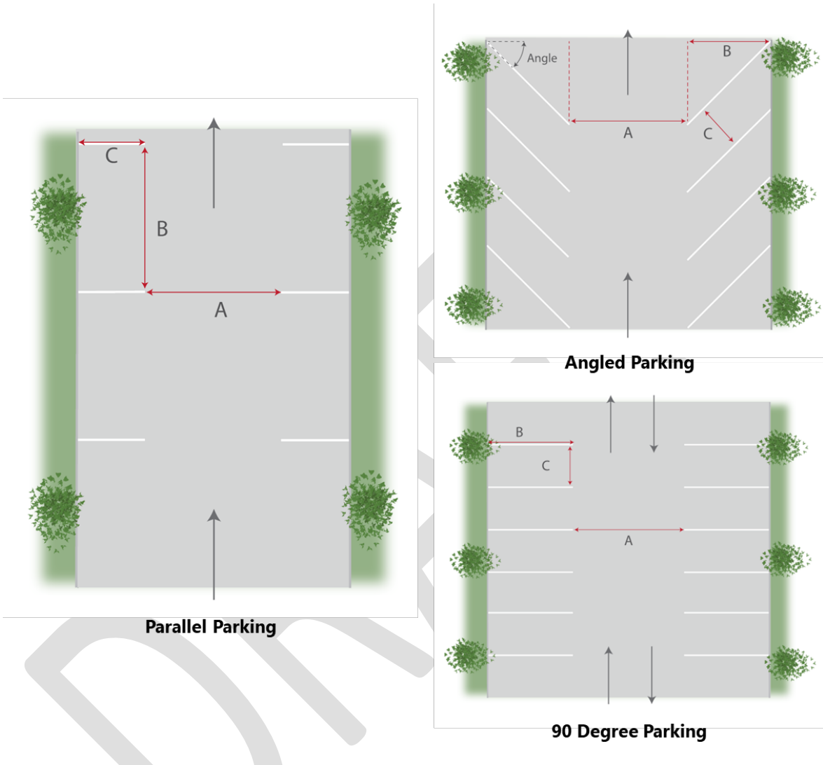
Figure 19.49.030: Parking Space and Aisle Dimensions.
