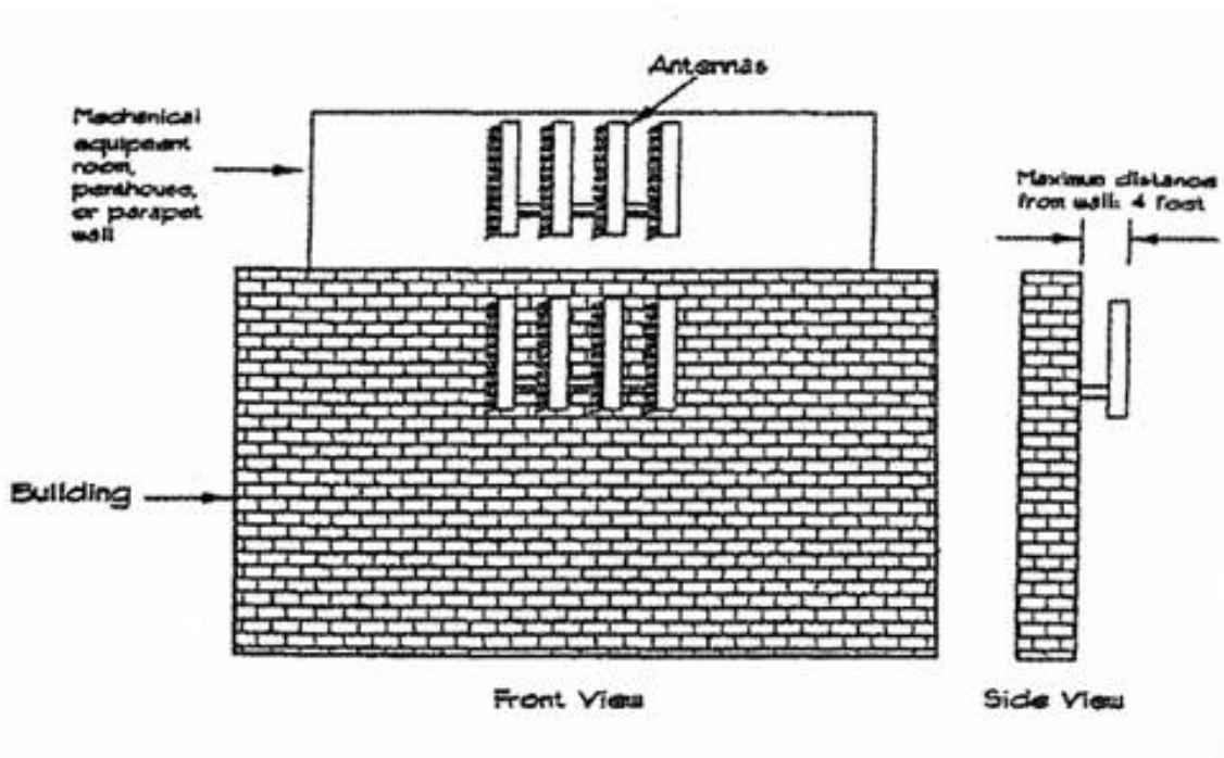
Figure 19.42.340B: Wall-Mounted Antennas.
