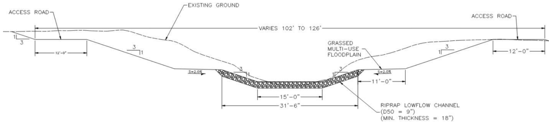
Figure 3-7. Pack Creek Preferred Cross Section
