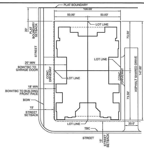
TYPICAL LOT CONFIGURATION SCALE 1"=80'
