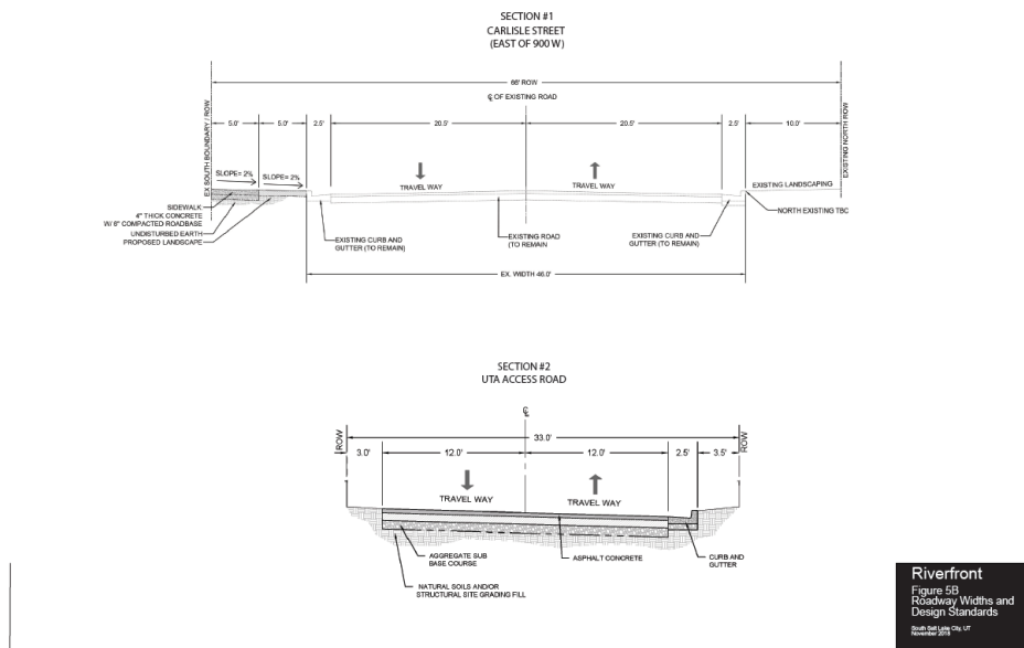
Figure 5B: Roadway Widths and Design Standards
