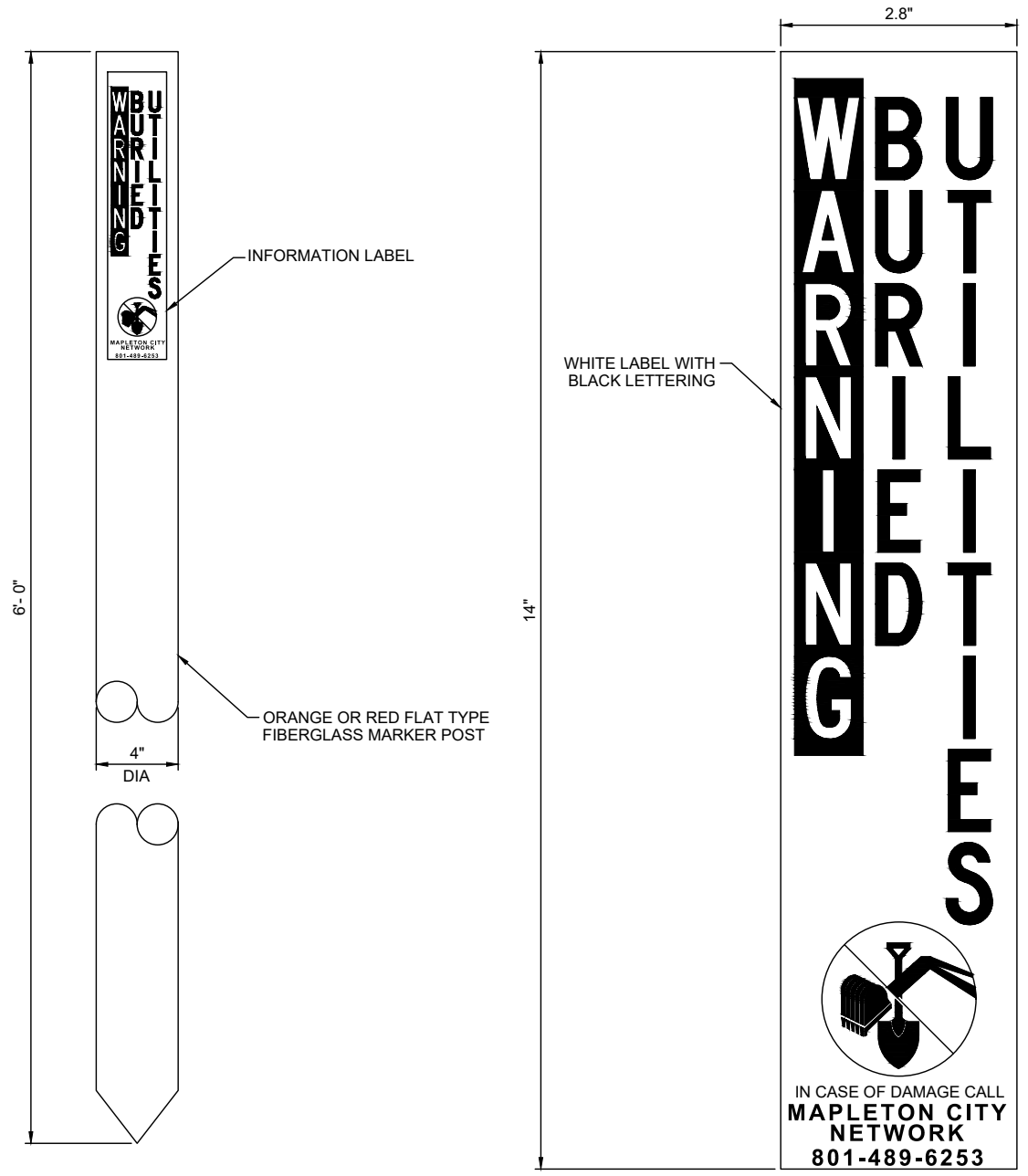
UTILITY MARKER POST - FLAT TYPE
