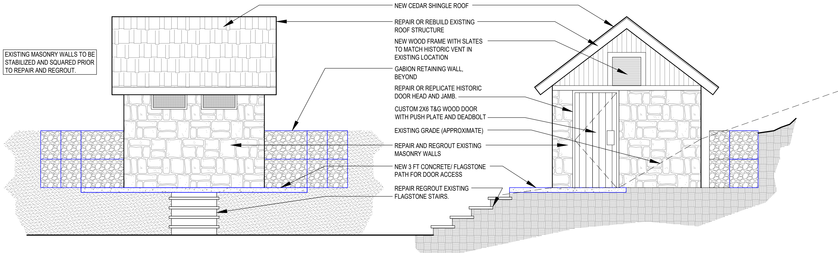
B FRONT ELEVATION DD-4 SCALE: 1/4"=1'-0"
