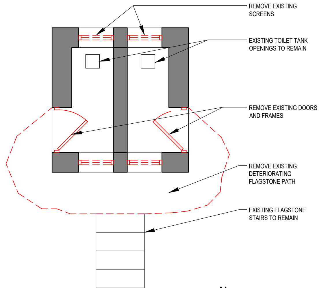
2 DD-3 DEMOLITION PLAN SCALE: 1/4"=1'-0"
