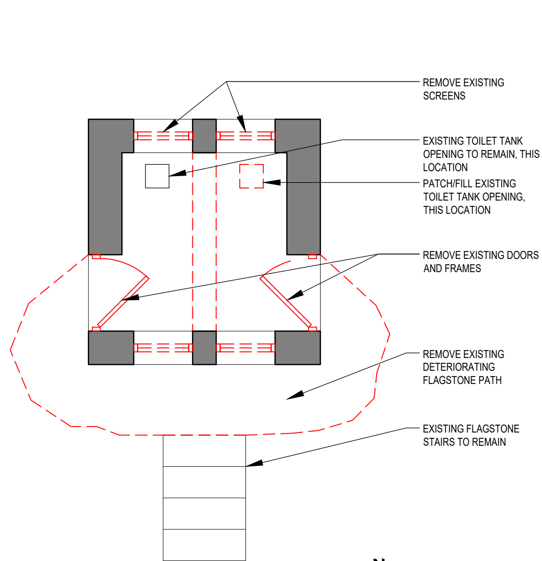
2 DD-2 DEMOLITION PLAN SCALE: 1/4"=1'-0"
