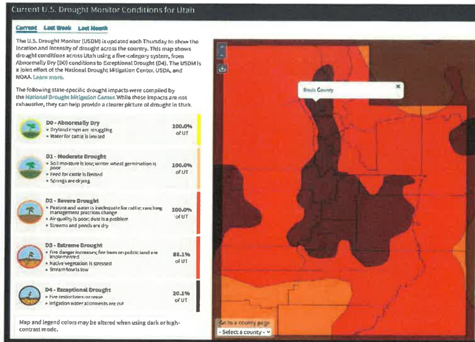
Figure 1 Drought Conditions 2021
