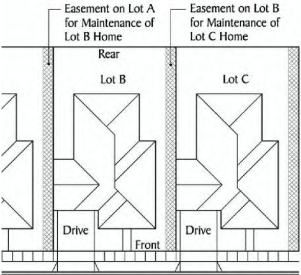
Zero lot line development Illustrative examples of some alternative lot configurations; not to scale
