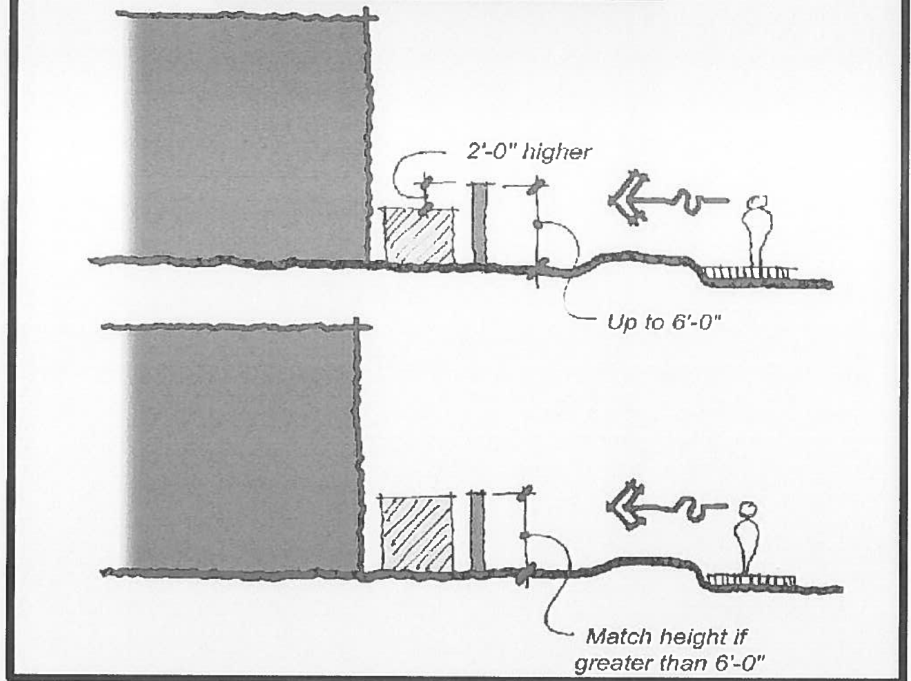
Figure 19-6 Ground Level Mech. Screening
