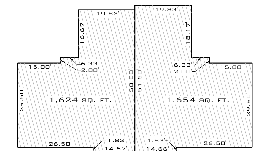
UNIT DIMENSION (TYPICAL): SCALE: 1"=15'
