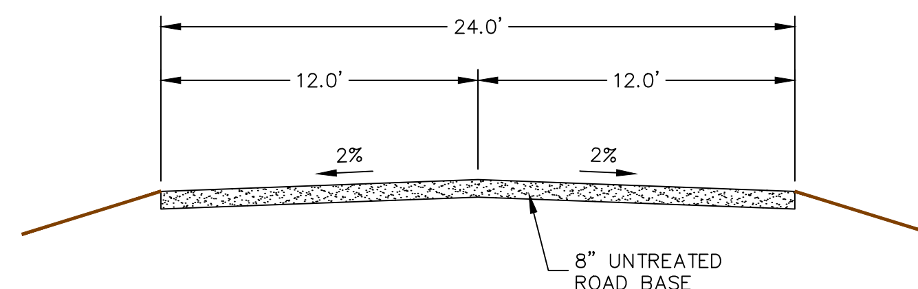
TEMPORARY UTILITY ACCESS ROAD - NTS -
