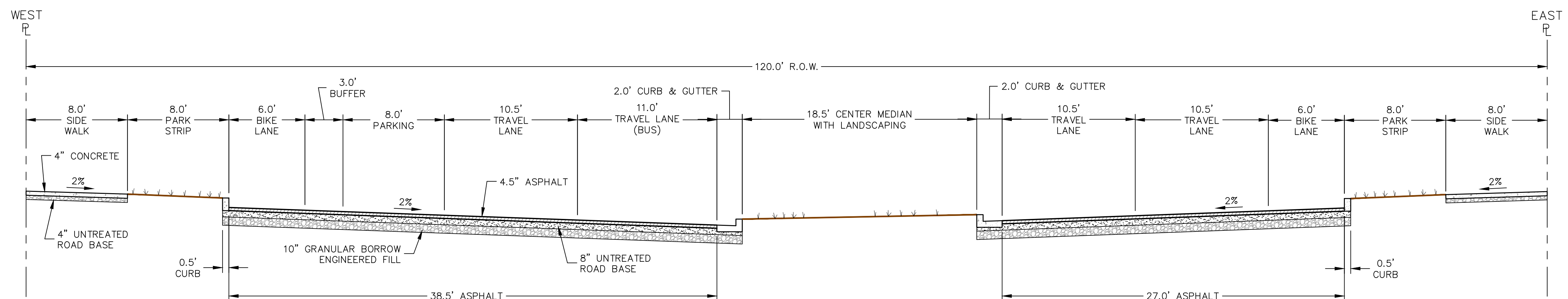
MAIN STREET BETWEEN SOUTH PROMENADE & AVENUE 1 - NTS -
