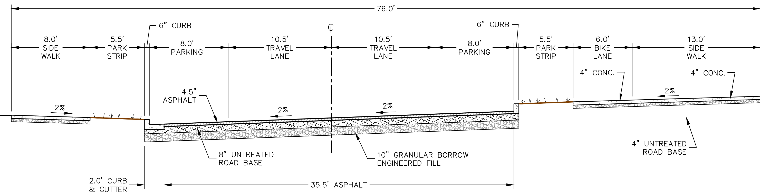
SOUTH SQUARE ABOUT (LOOKING EAST) - NTS -
