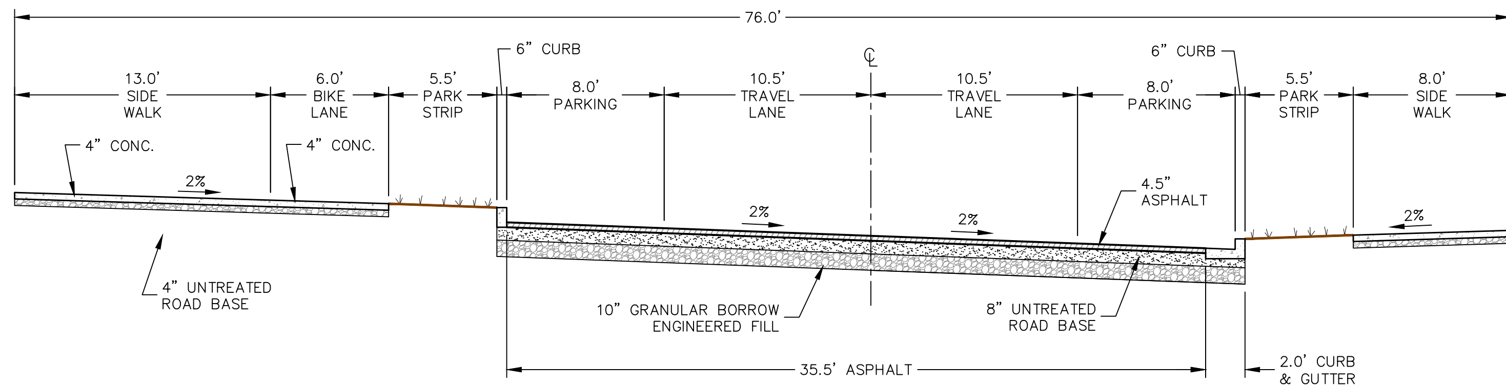
NORTH SQUARE ABOUT (LOOKING EAST) - NTS -
