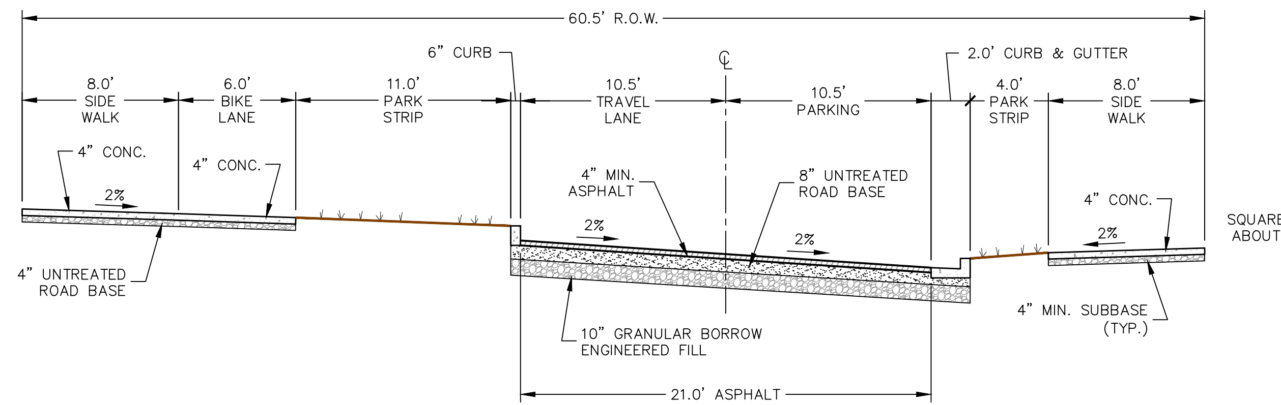
WEST SQUARE ABOUT (LOOKING NORTH) - NTS -
