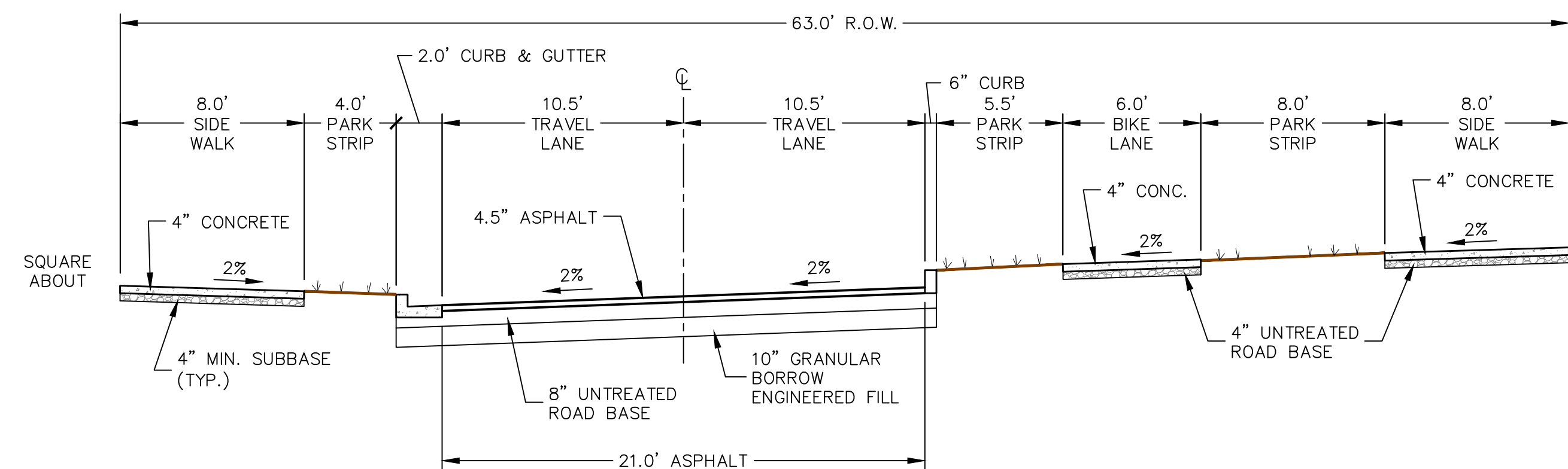
EAST SQUARE ABOUT (LOOKING NORTH) - NTS -
