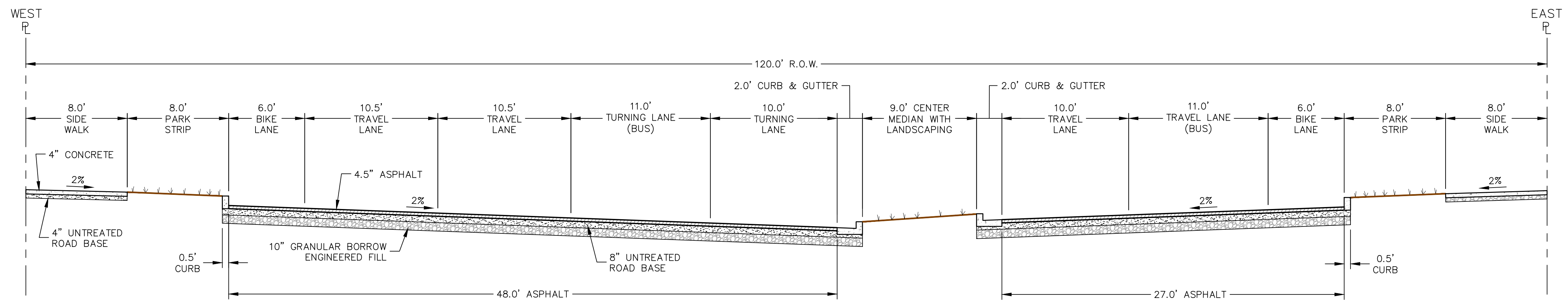
MAIN STREET BETWEEN AVENUE 1 & VINEYARD CONNECTOR - NTS -
