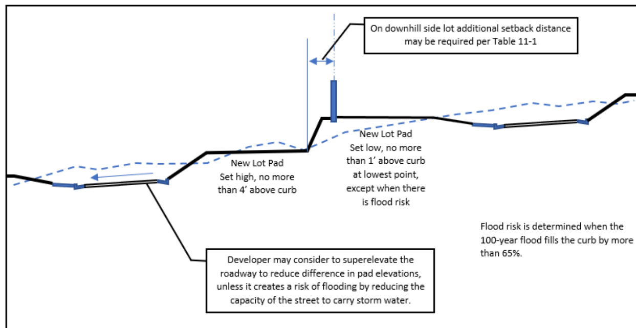
Figure 11-10 - Grading residential pads on the interior of the subdivision to reduce grade differences.
