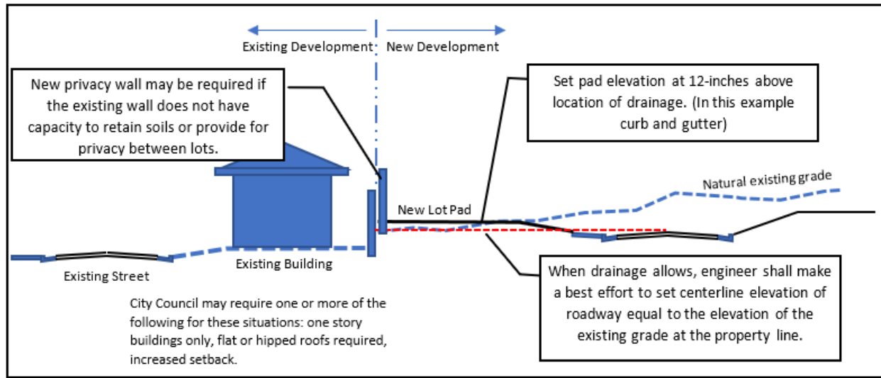
Figure 11-6 Developing on Slopes – Grading residential pads next to a property on the downhill side of the development adjacent to existing development
