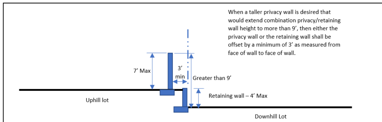
Figure 11-12 – Side Lot Retaining Walls/Privacy Walls
