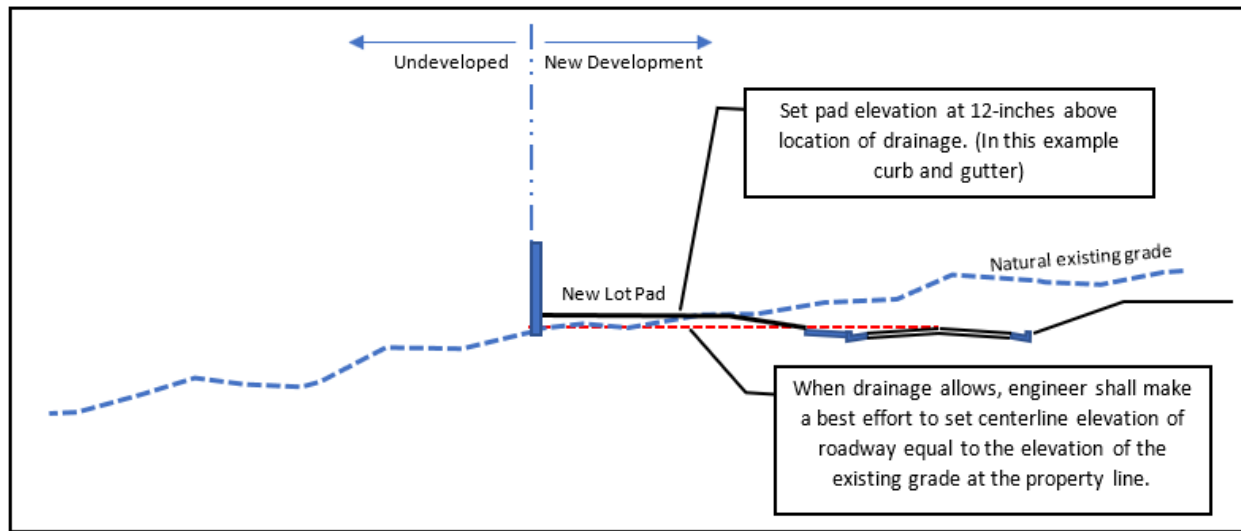
Figure 11-7 Developing on Slopes – Grading residential pads next to a property on the downhill side of the development adjacent to undeveloped property
