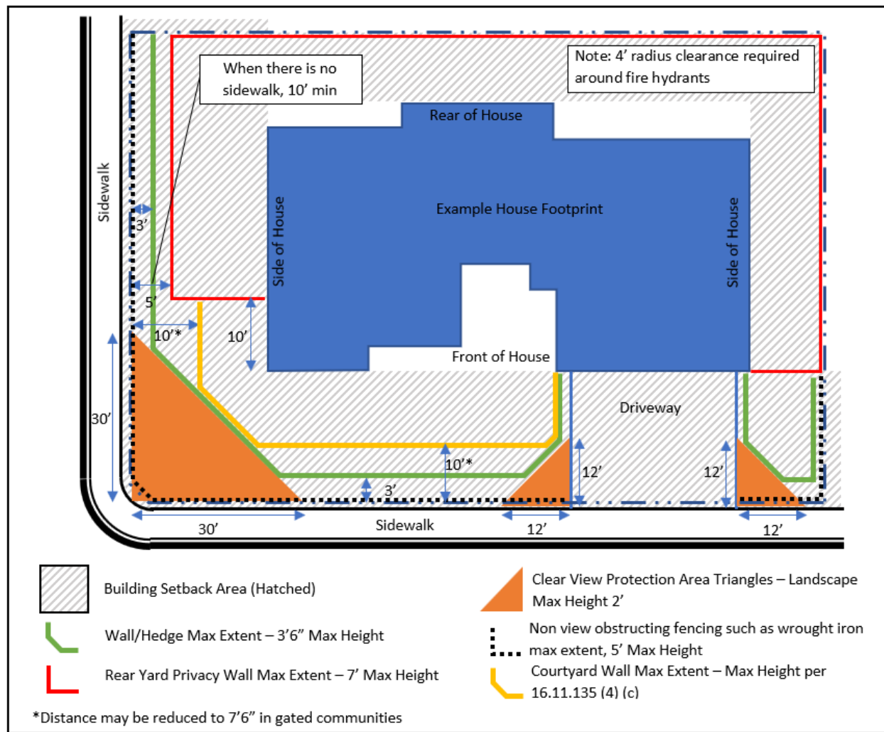
Figure 11-14 – Corner Lot Example – Maximum Wall Extents Allowable
