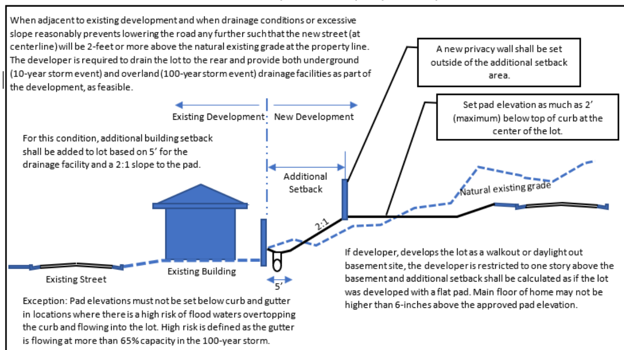
Figure 11-8 - Developing on Slopes – Grading residential pads next to a developed property on the downhill side of the development – steep slopes example
