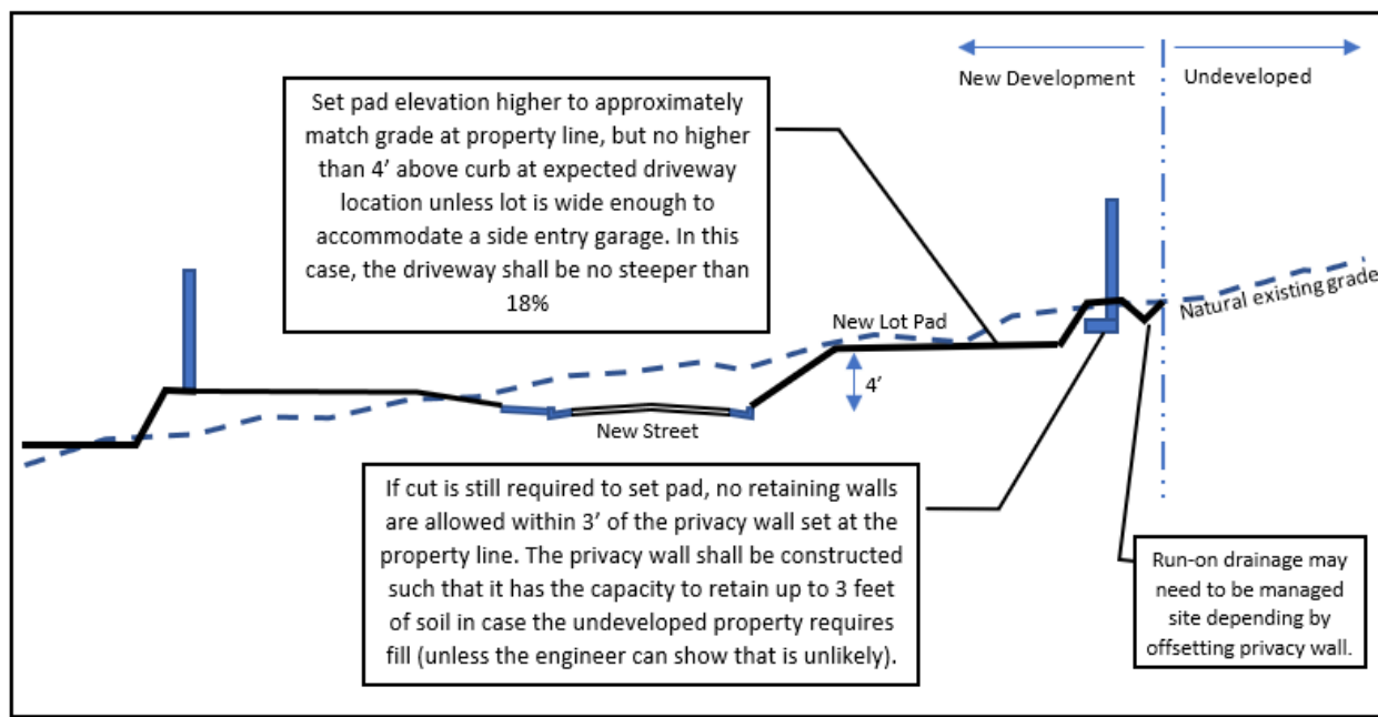
Figure 11-9 - Developing on Slopes – Grading residential pads next to an undeveloped property on the uphill side of the development
