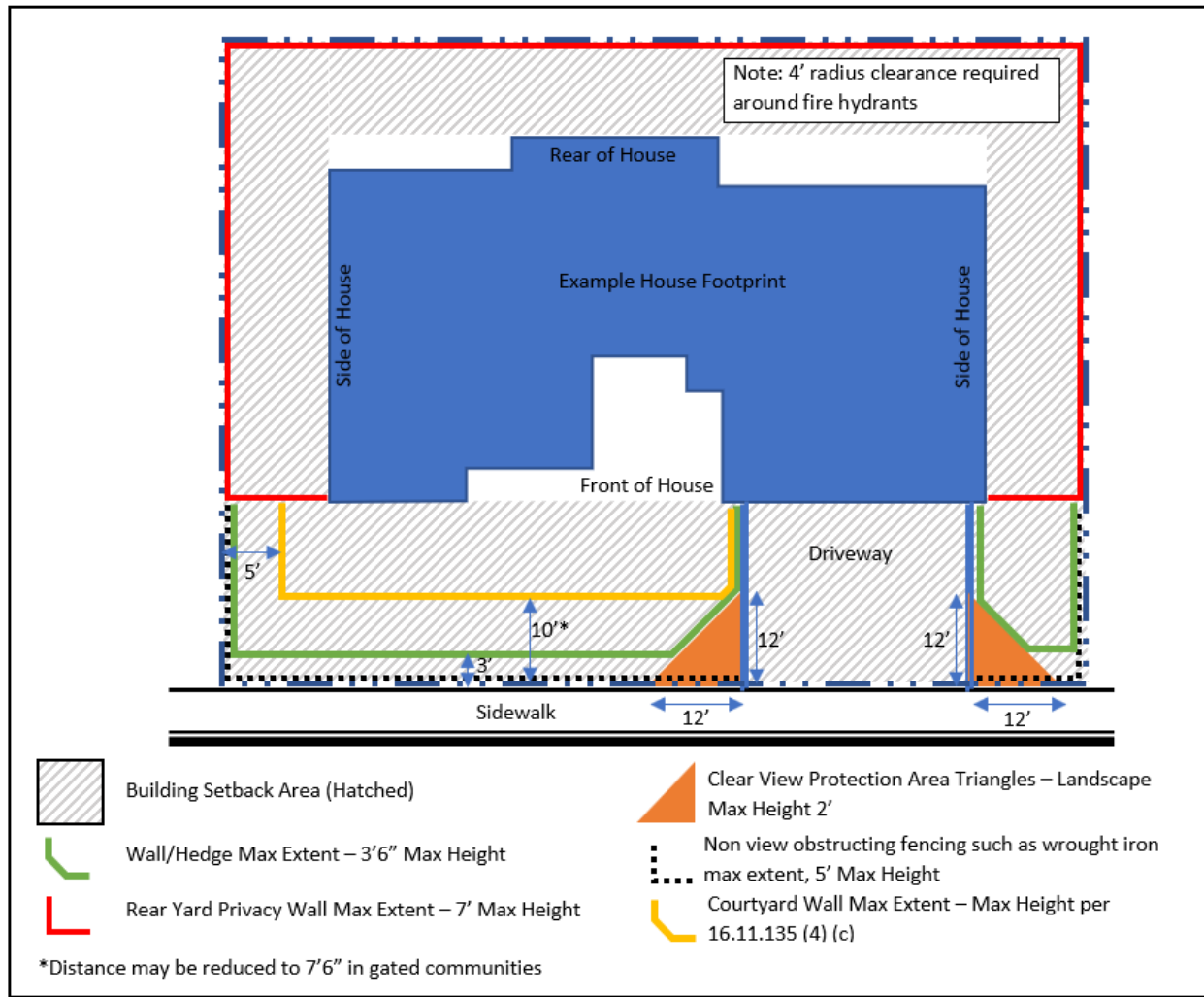
Figure 11-11 – Interior Lot Example – Maximum Wall Extents Allowable
