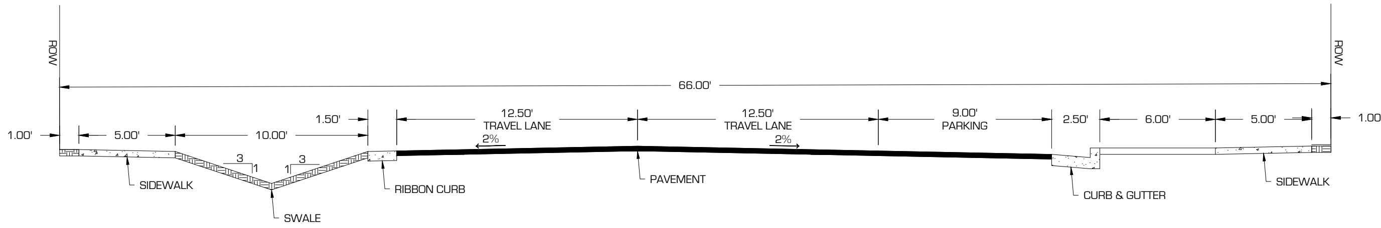
MODIFIED TS-14 #1 NOT TO SCALE
