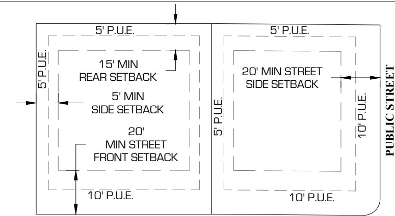
PUE & SETBACK DETAIL (TYPICAL SEE DRAWING FOR EXCEPTIONS) NTS
