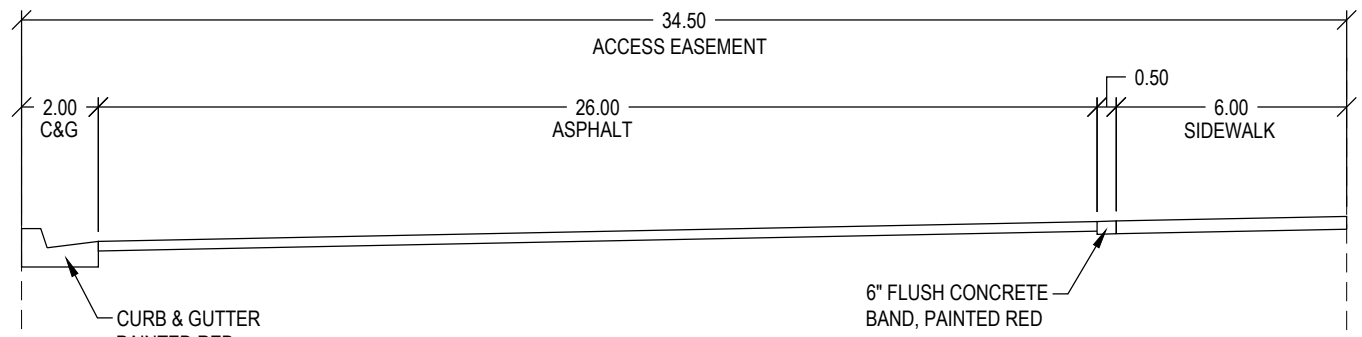
PRIVATE ROAD - SECTION VIEW
