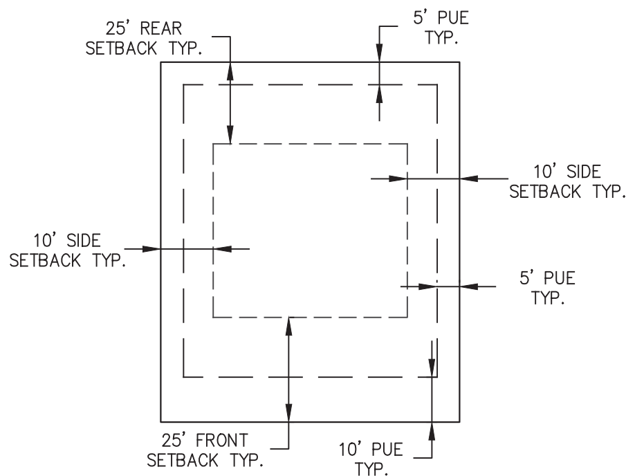
DETAIL-TYP. BUILDING SETBACK AND EASEMENT -NTS-
