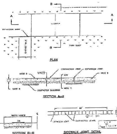
Concrete sidewalk
