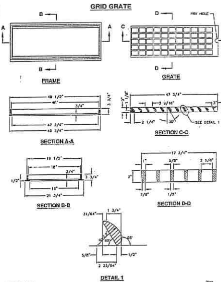
47 3/4" Grate end frame
