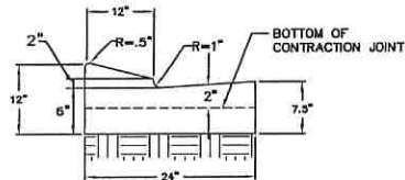
TYPE B-CURB DETAIL -NTS-
