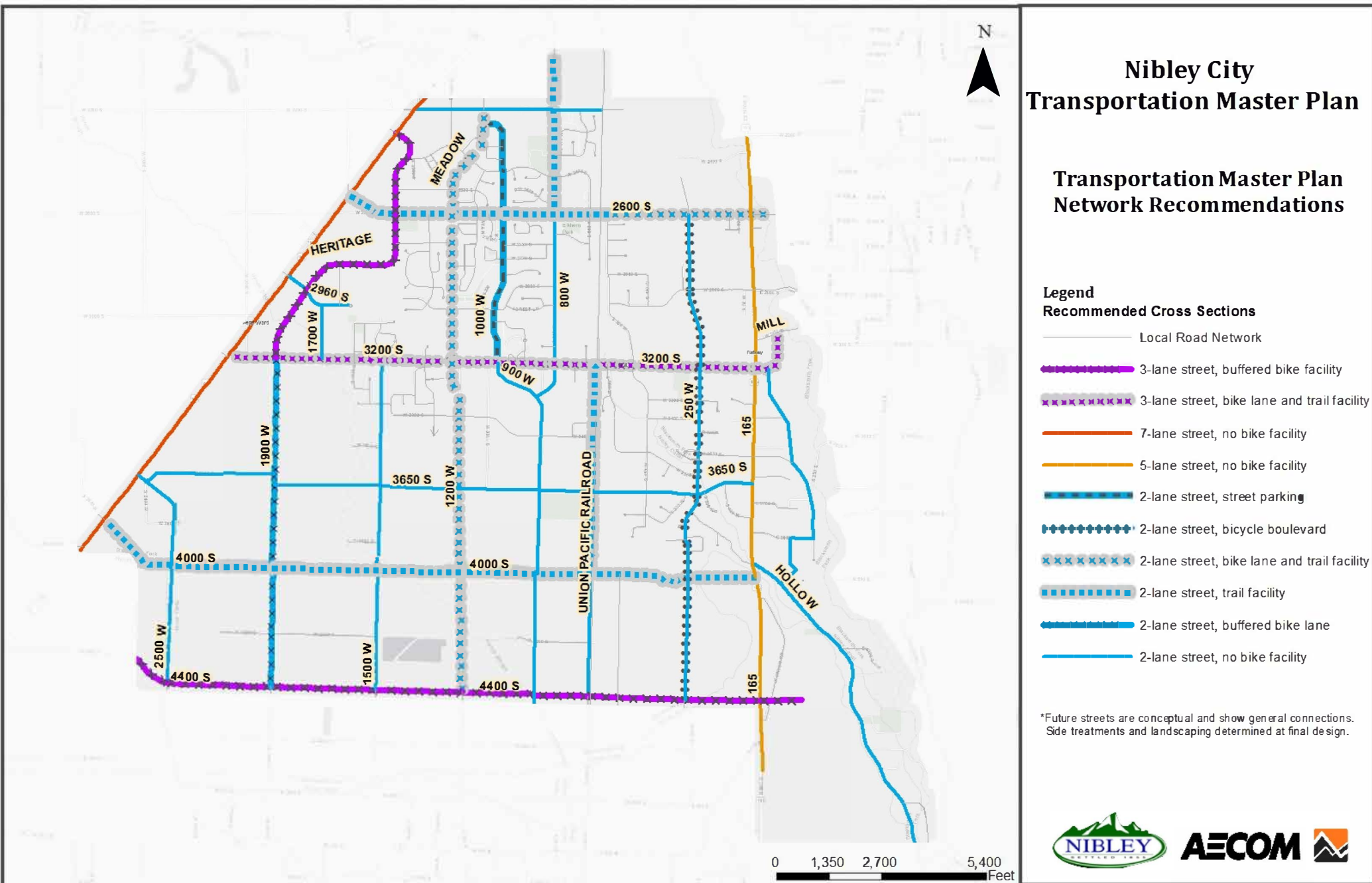
FIGURE 1: RECOMMENDED STREET NETWORK
