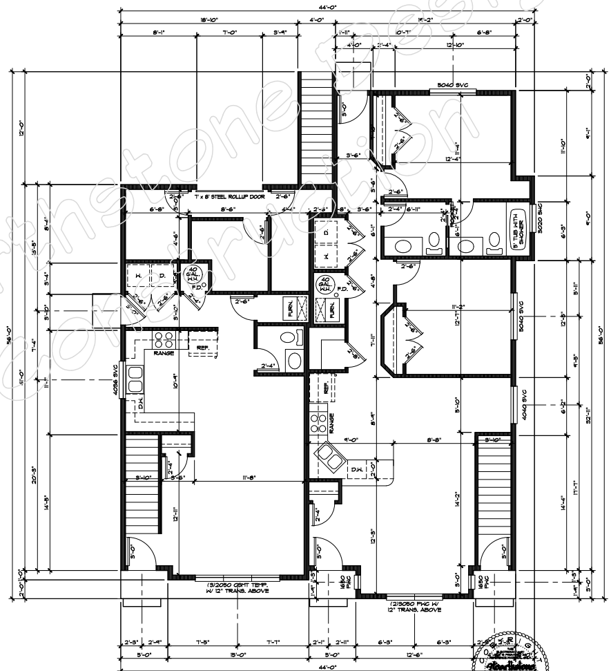
MAIN FLOOR PLAN SCALE: 1/4"=1'-0" UNIT 1: 1,186 S.F. UNIT 2: 1,169 S.F.
