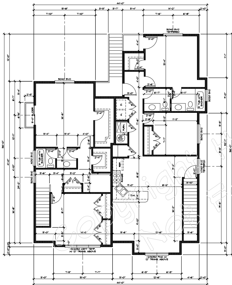
UPPER FLOOR PLAN SCALE: 1/4"=1'-0" UNIT 1: 1,186 S.F. UNIT 2: 1,169 S.F.
