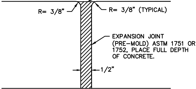
EXPANSION JOINT
