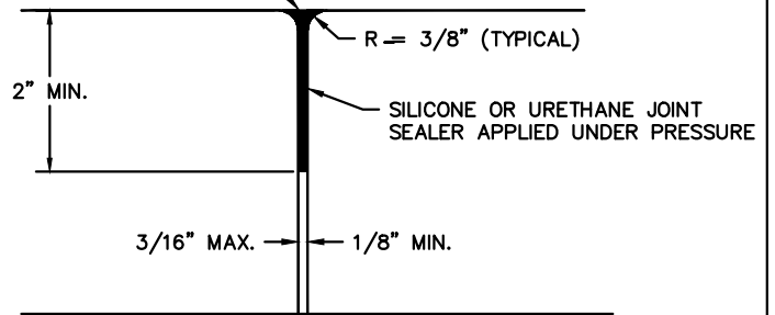
FORM PLATE JOINT
