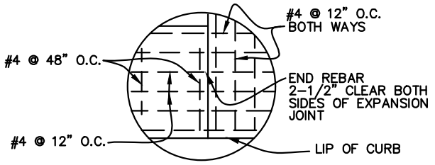
REINFORCING DETAIL
