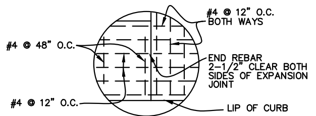
REINFORCING DETAIL
