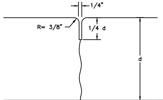
CONTROL JOINT
