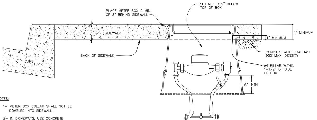
SECTION
