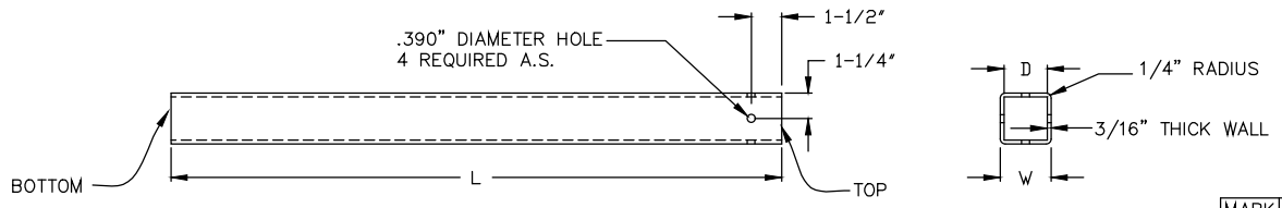
SIGN ANCHOR DETAIL
