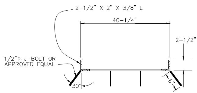
SECTION C-C
