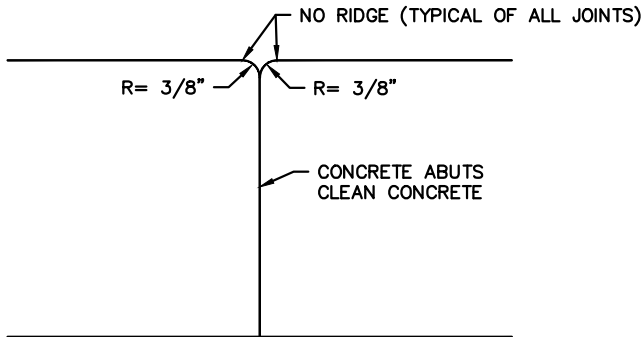
COLD JOINT
