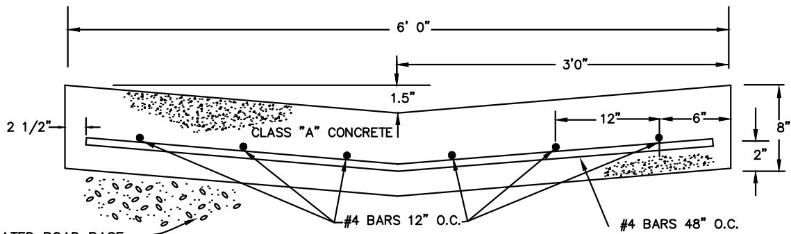
6' CROSS SECTION
