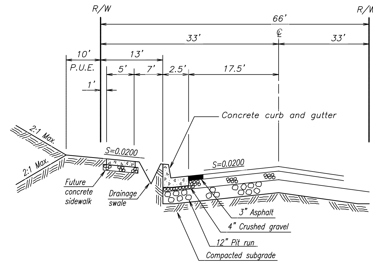
TYPICAL 66' STREET SECTION NO SCALE
