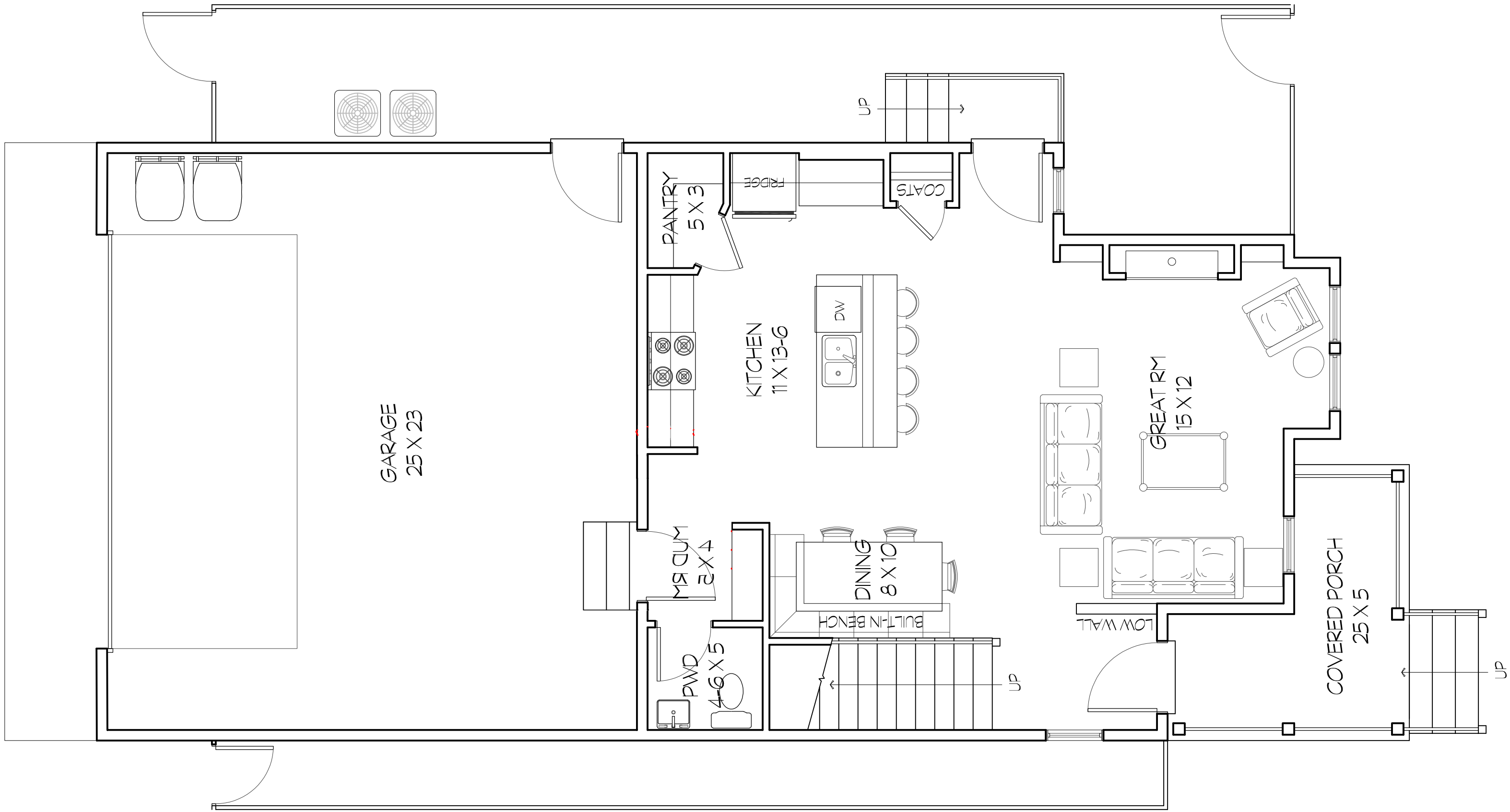
PH3 LEVEL 1 1384 SqFt Gross (including garage & porch) 635 SqFt Net (livable)
