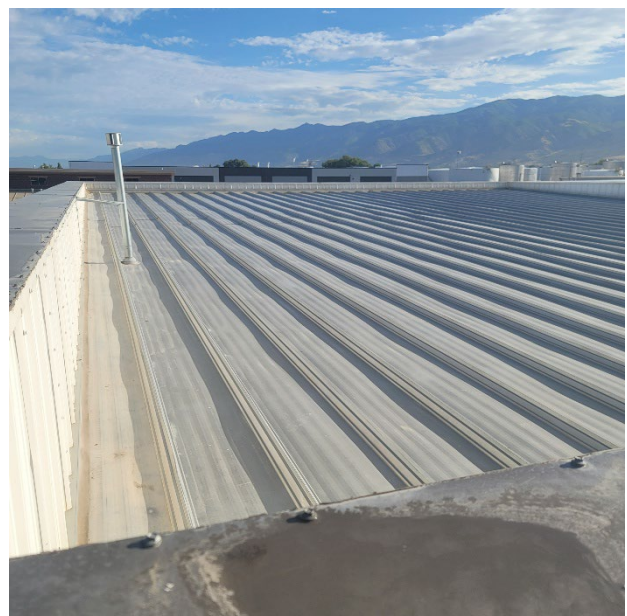
Figures 7 & 8 - Galvanized metal roofs routinely leak at top parapet walls, side parapet walls, and at the gutter adjoining the bottom parapet wall.
