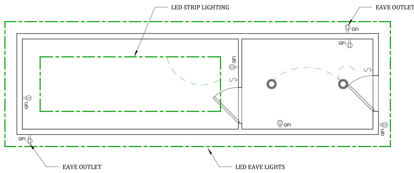
Electrical Plan
