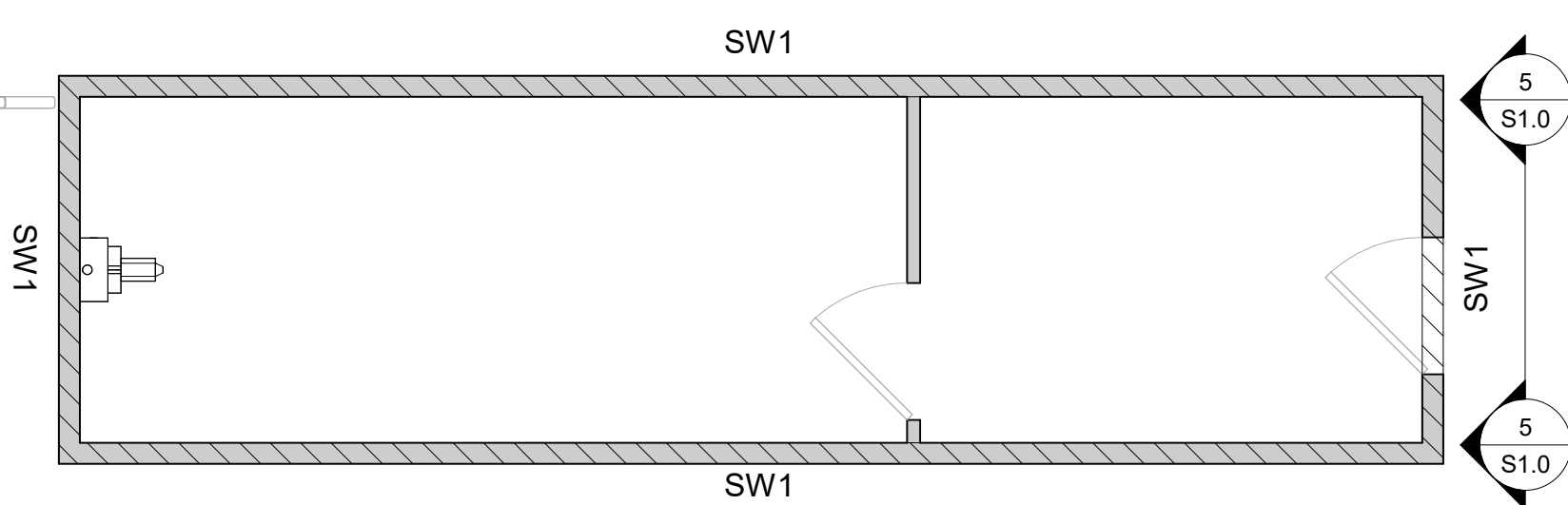
Main Floor Shear Wall Plan
