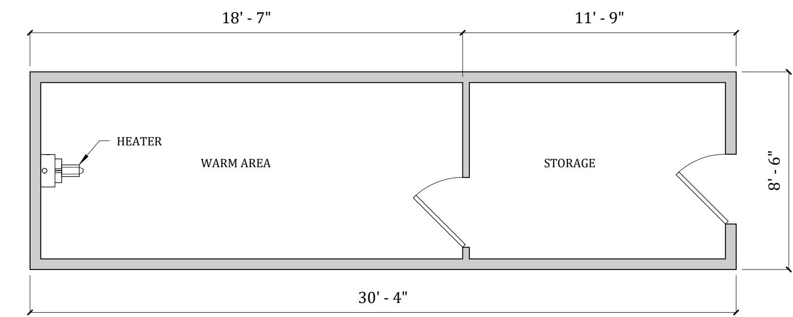
Building Layout
