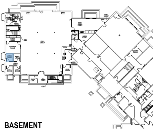
BASEMENT
