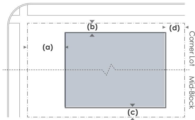
PRINCIPLE BUILDING SETBACKS
