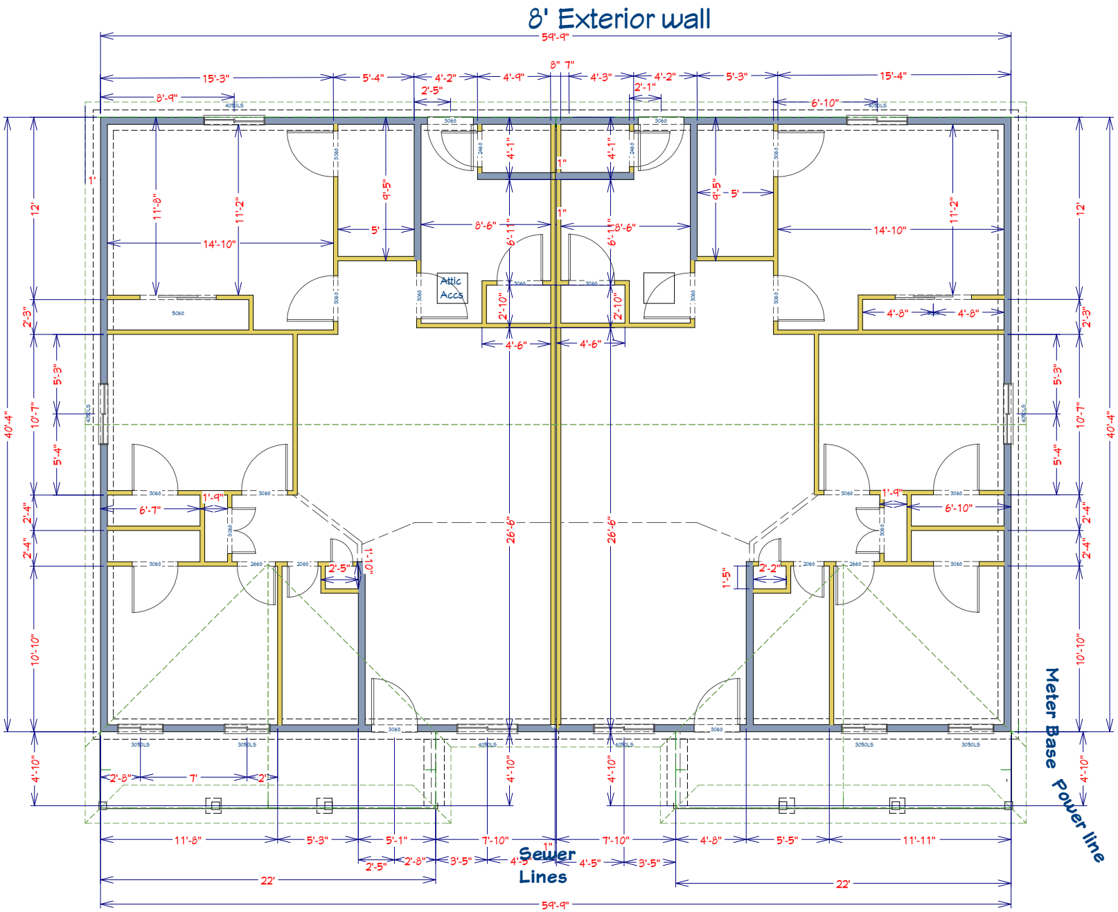
Framing plan
