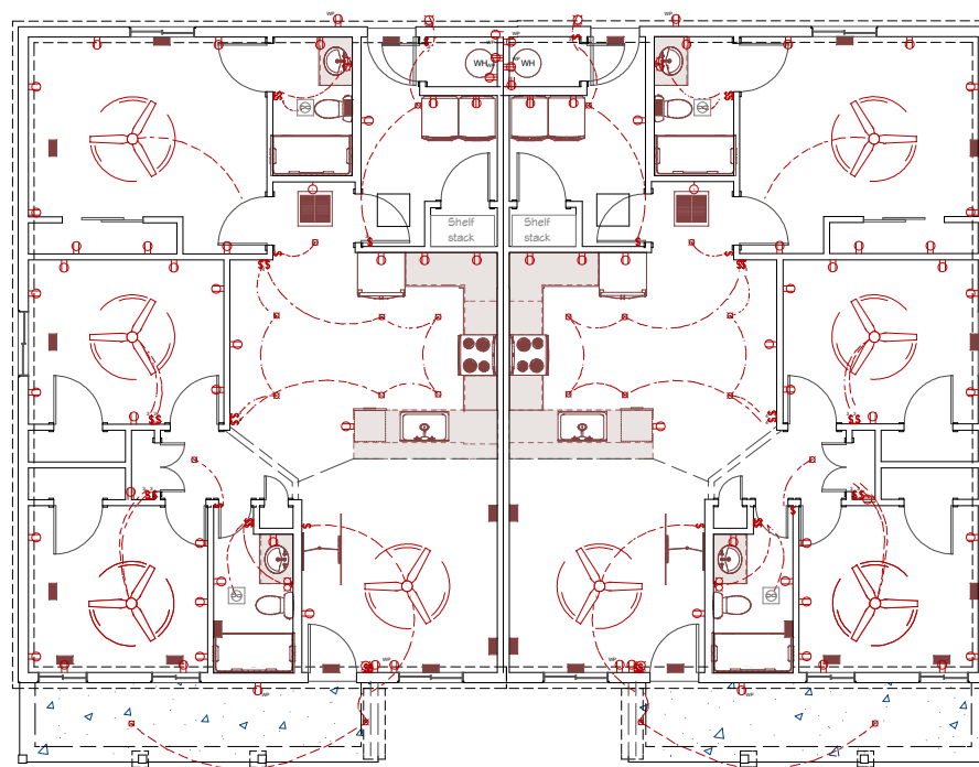
Electrical Plan
