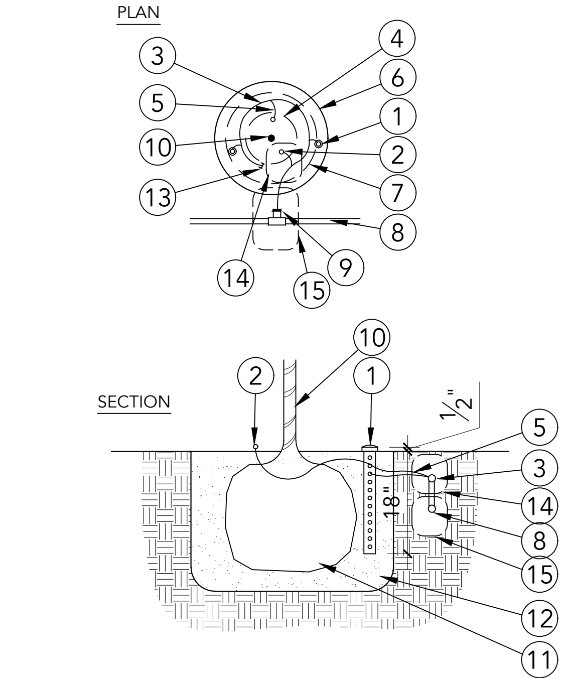
G DRIP EMITTER FOR TREE SCALE: 3" = 1'-0"
