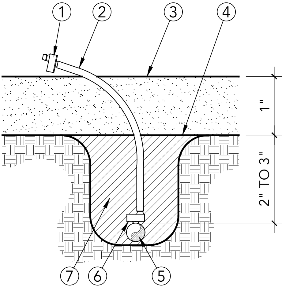
F EMITTER CONNECTION TO XERI-TUBE SCALE: 6" = 1'-0"
