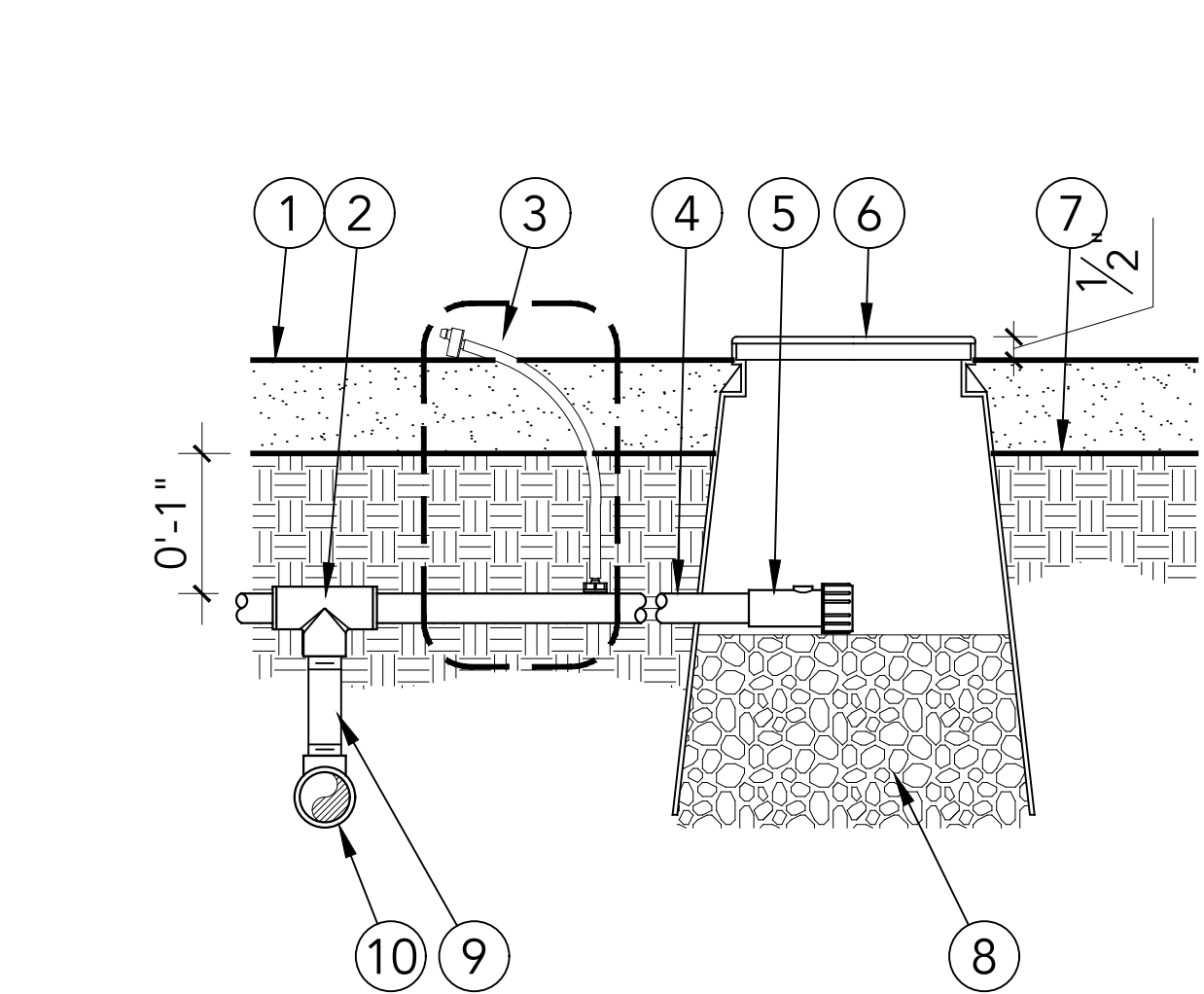
H PVC TO TUBING CONNECTION SCALE: 3" = 1'-0"
