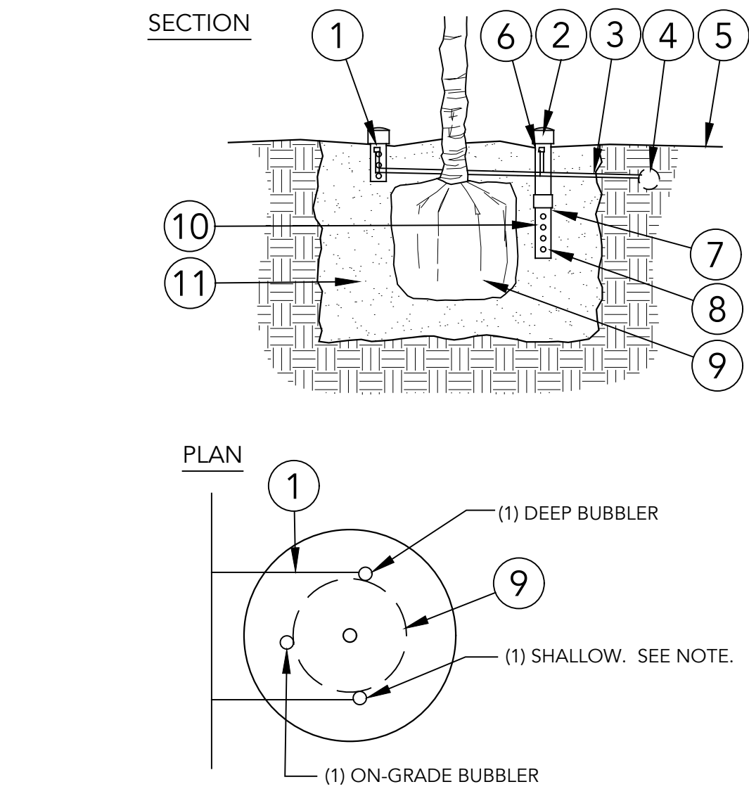
I BUBBLERS - PALM AND LARGE TREES SCALE: 3" = 1'-0"
