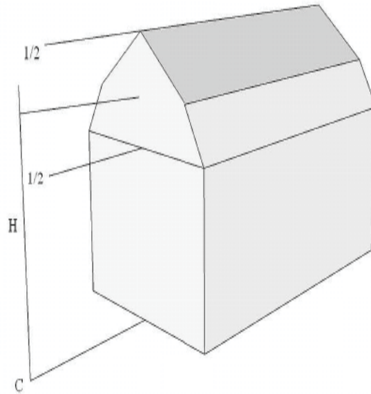
GAMBREL ROOF
