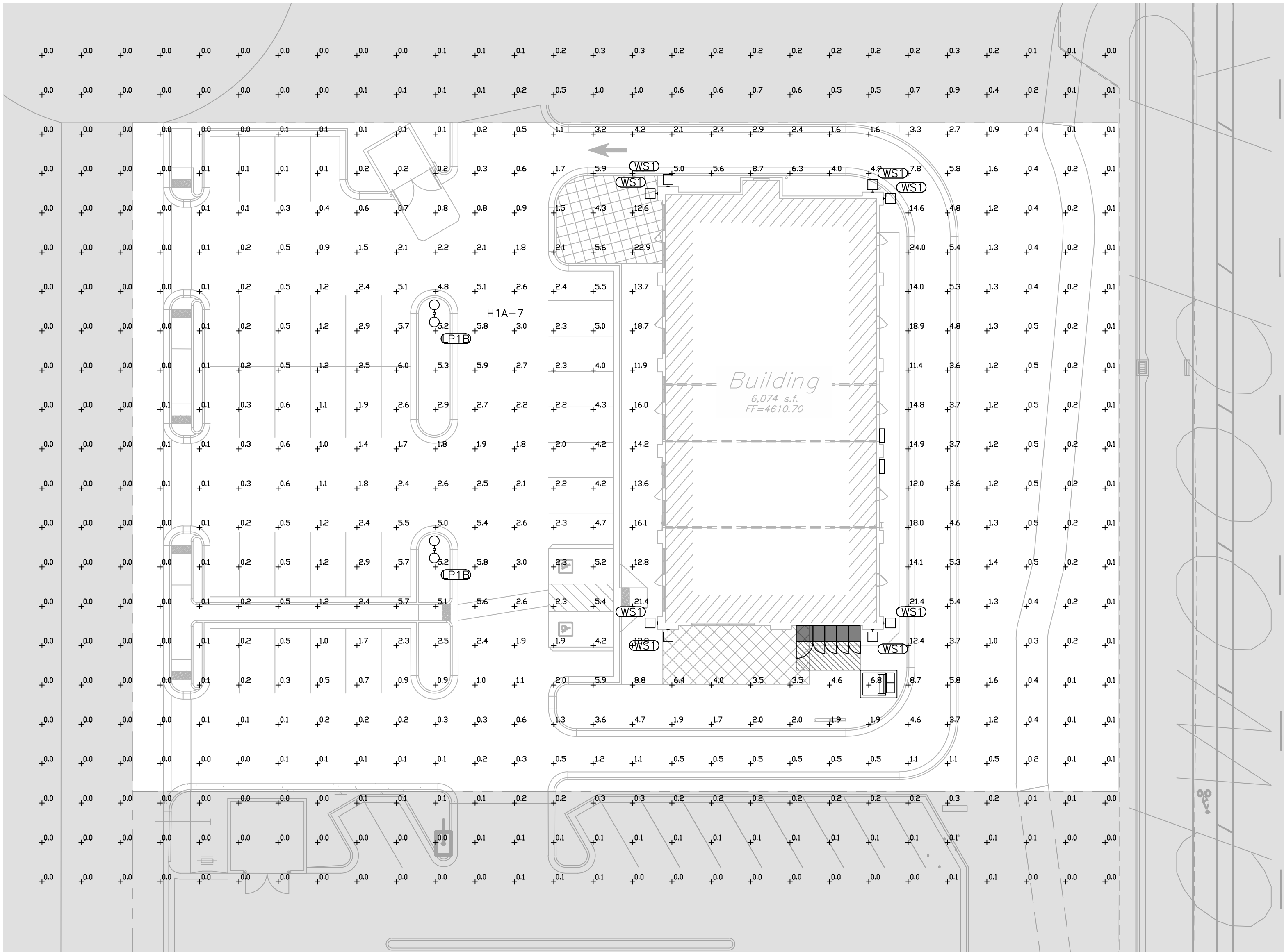
1 ELECTRICAL SITE PHOTOMETRIC PLAN SCALE: 1" = 20'-0"
