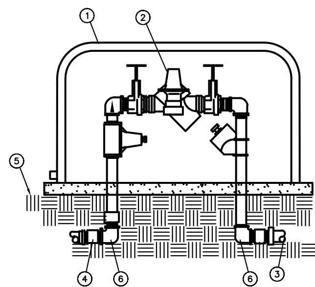
D REDUCED PRESSURE BACKFLOW VALVE N.T.S.
