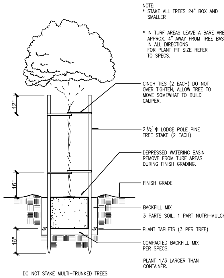
B TREE PLANTING W/ DOUBLE STAKING N.T.S.
