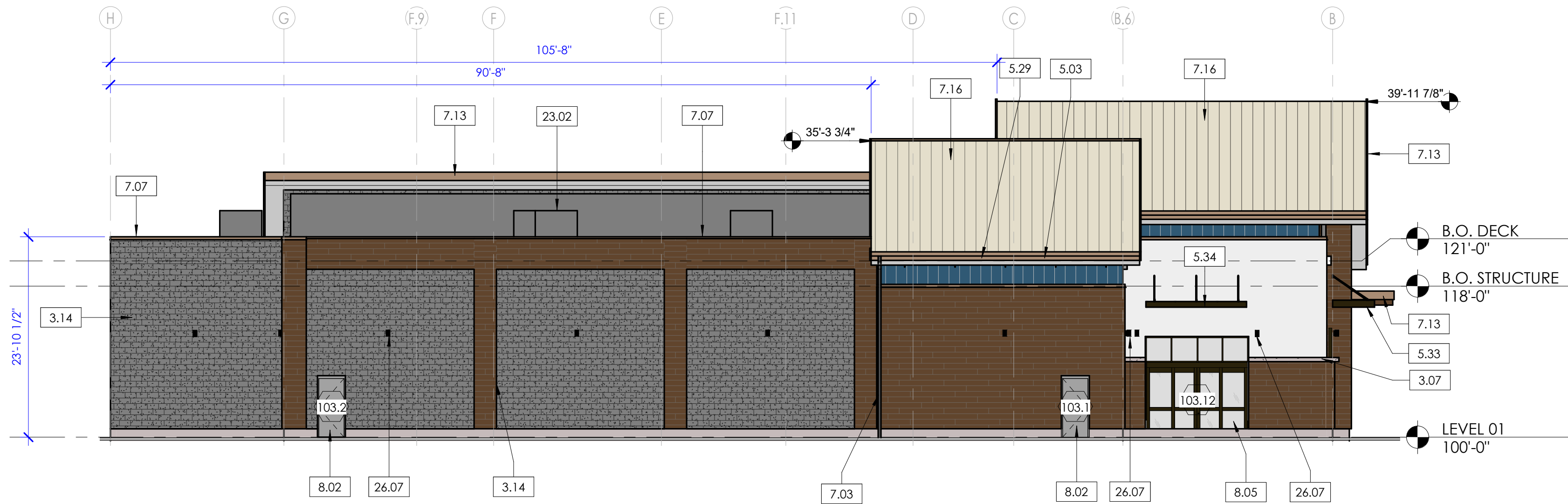
B3 A201 WEST ELEVATION 3/32" = 1'-0"
