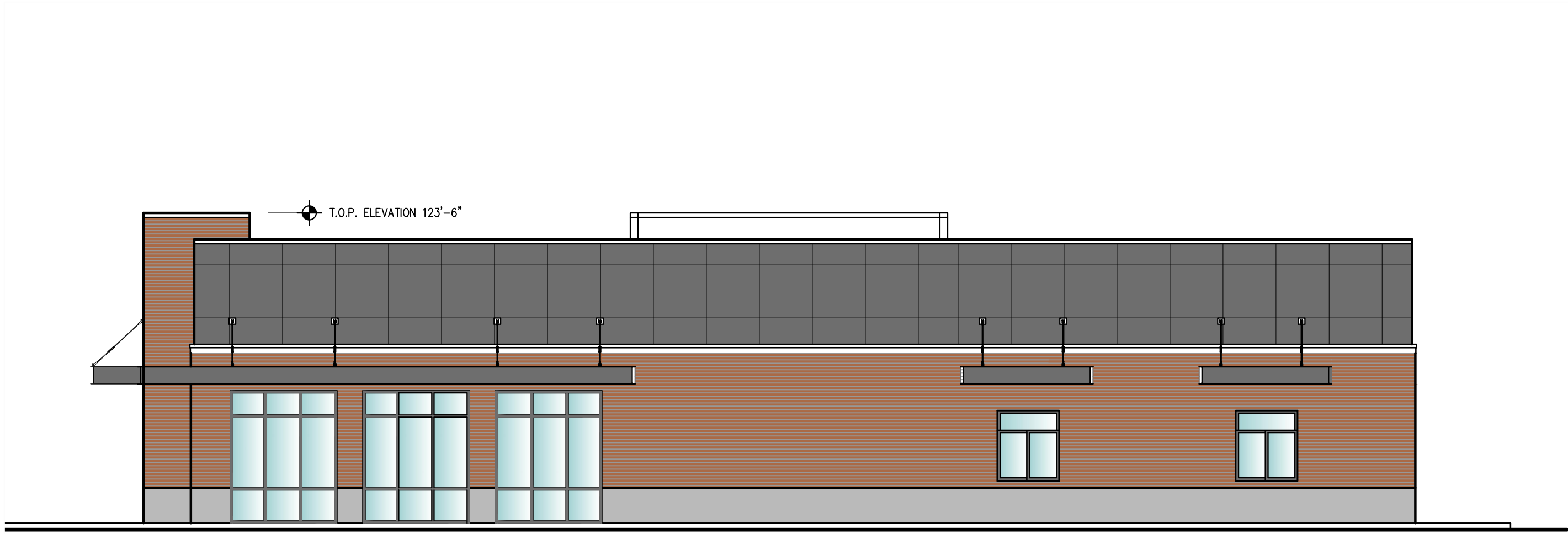
SIDE ELEVATION - SOUTH SCALE: 1/8" = 1'-0"
