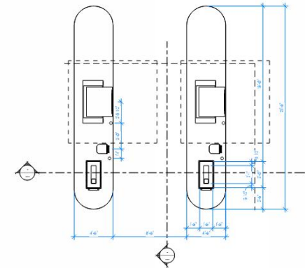
6 MAIN LEVEL 1/8" = 1'-0"
