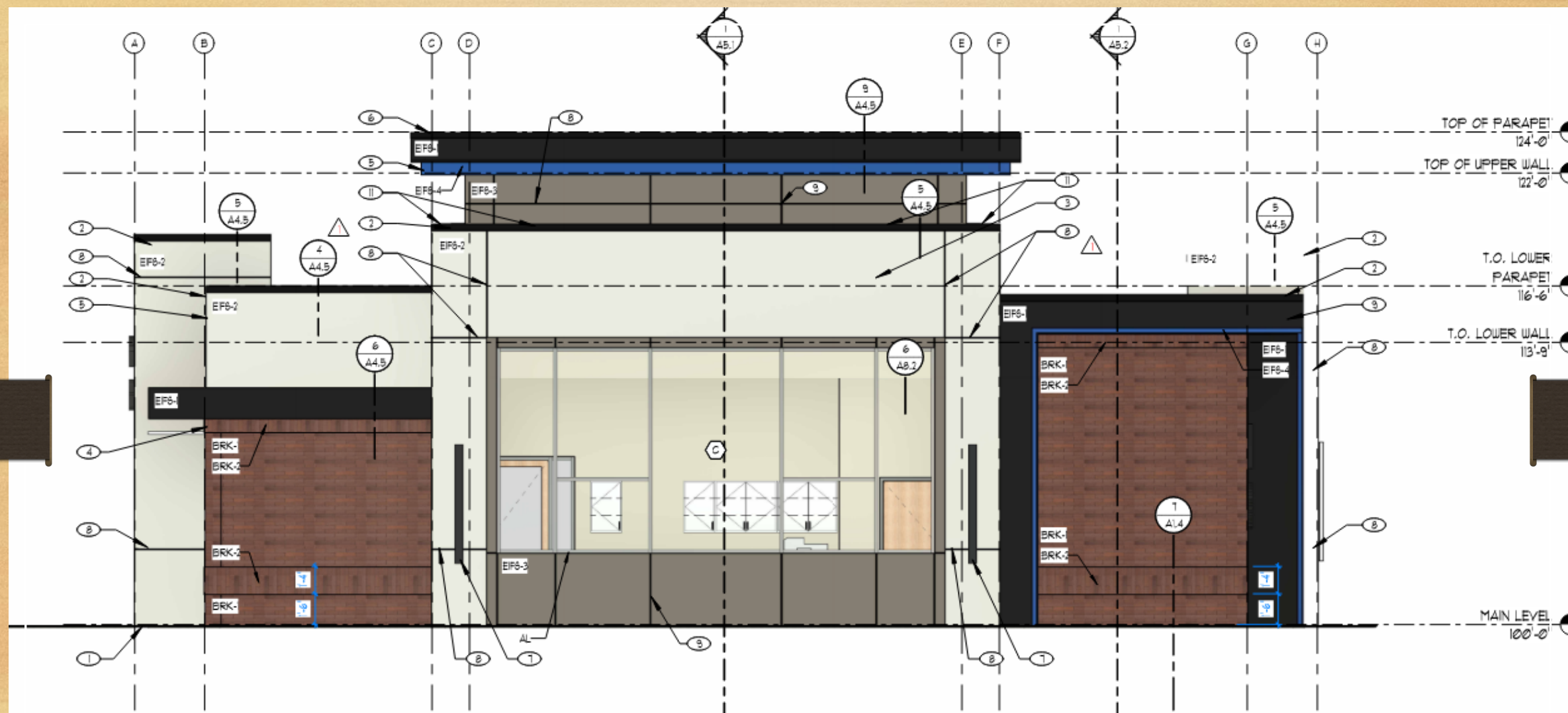
2 WEST ELEVATION 1/4" = 1'-0"
