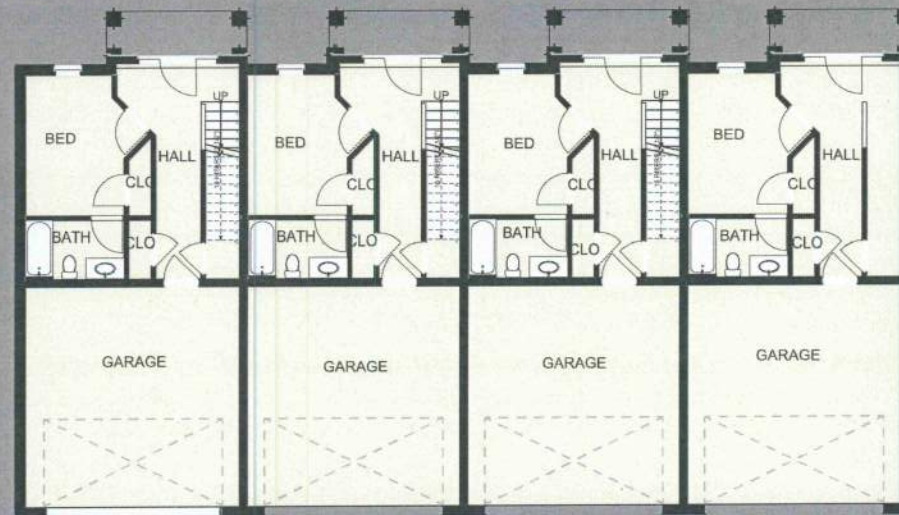
3-story Options - GROUND FLOOR PLAN
