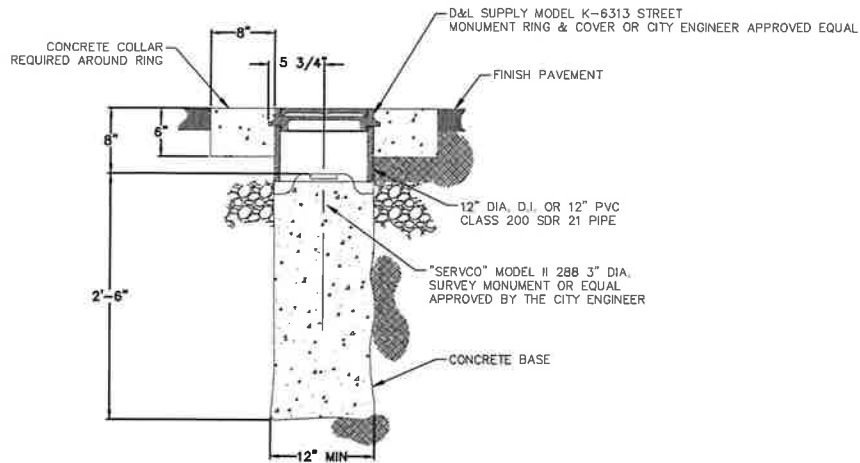
SURVEY MONUMENT SECTION
