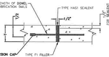
TYPE D JOINT
