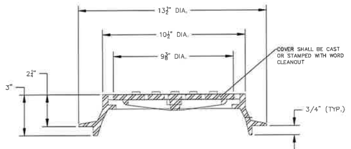
STANDARD CLEANOUT RING & LID (H-20 RATING)
