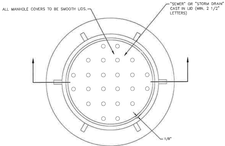
PLAN OF COVER & FRAME
