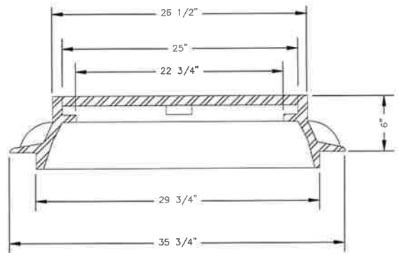
SECTION 1
