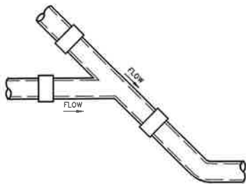
DETAIL - DROP C.O. (WHERE REQUIRED)
