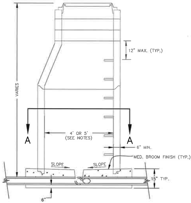
TYPICAL JUNCTION MANHOLE (SECTION THRU CENTER)
