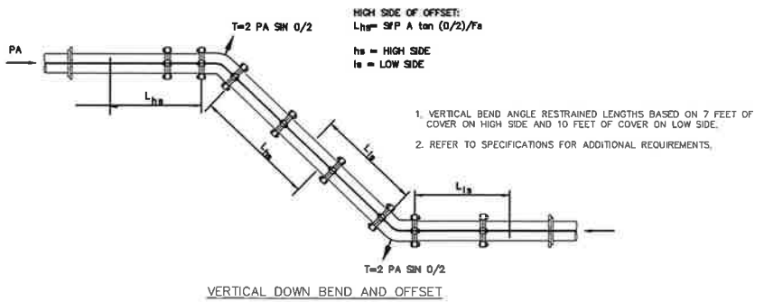
VERTICAL DOWN BEND AND OFFSET
