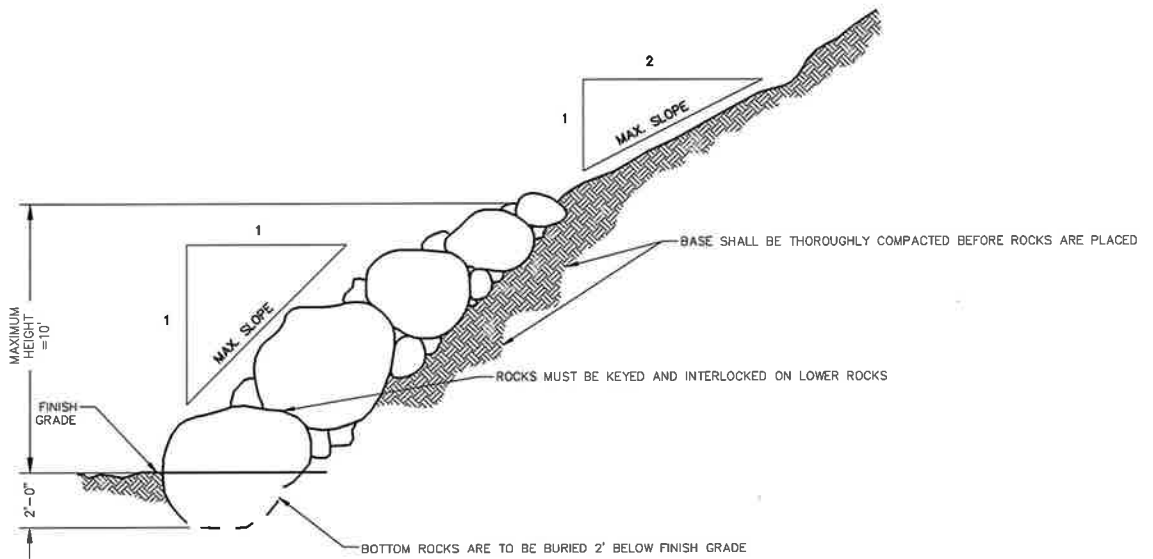
CROSS SECTION
