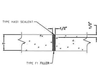
TYPE G JOINT
