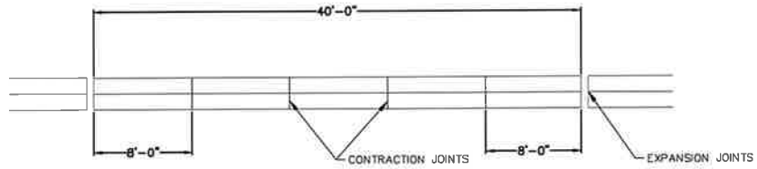
CURB AND GUTTER DETAIL
