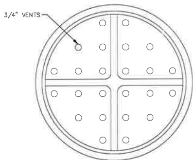
BOTTOM VIEW OF COVER
