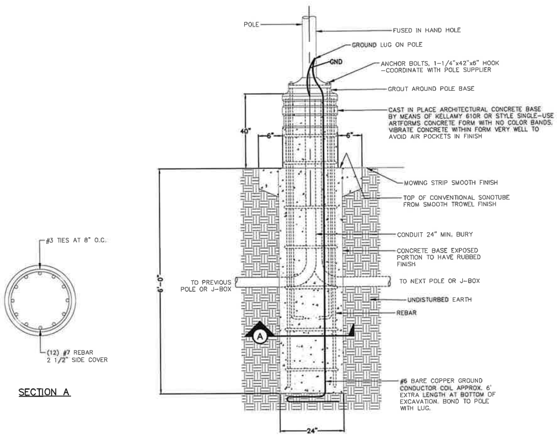
SMALL AREA LIGHTING POLE MOUNTING DETAIL
