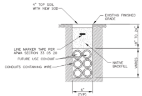
A1 LANDSCAPE TRENCH DETAIL SCALE: NTS
