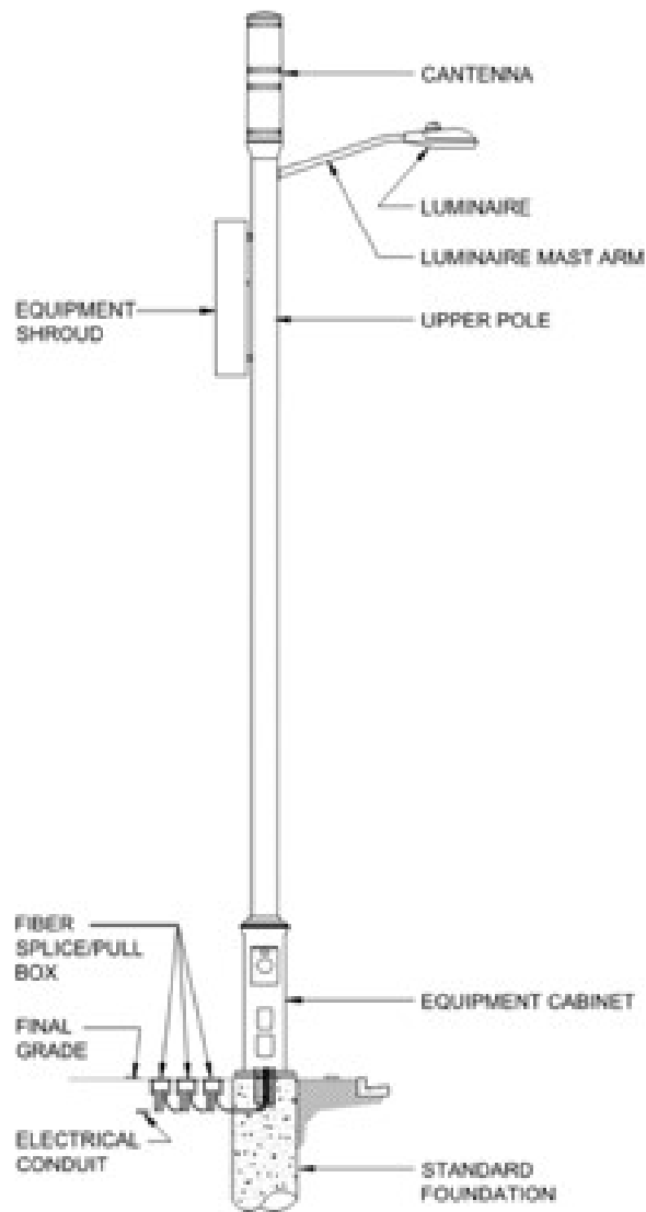
Figure 5-4: Combination Street Light Pole with Antenna and Equipment Shroud
