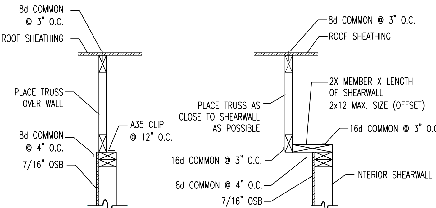
2 INTERIOR SHEARWALL TO TRUSS CONNECTION S102, S103 N.T.S.
