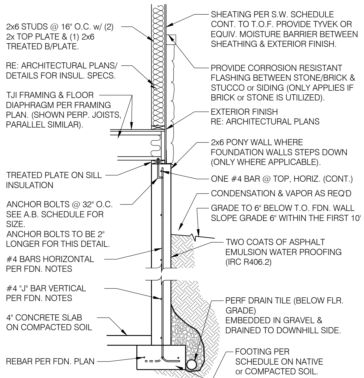
5 TYP. WALL SECTION (SIDING / STUCCO / CULT. STONE) 2x SCALE LISTED IN TITLEBLOCK
