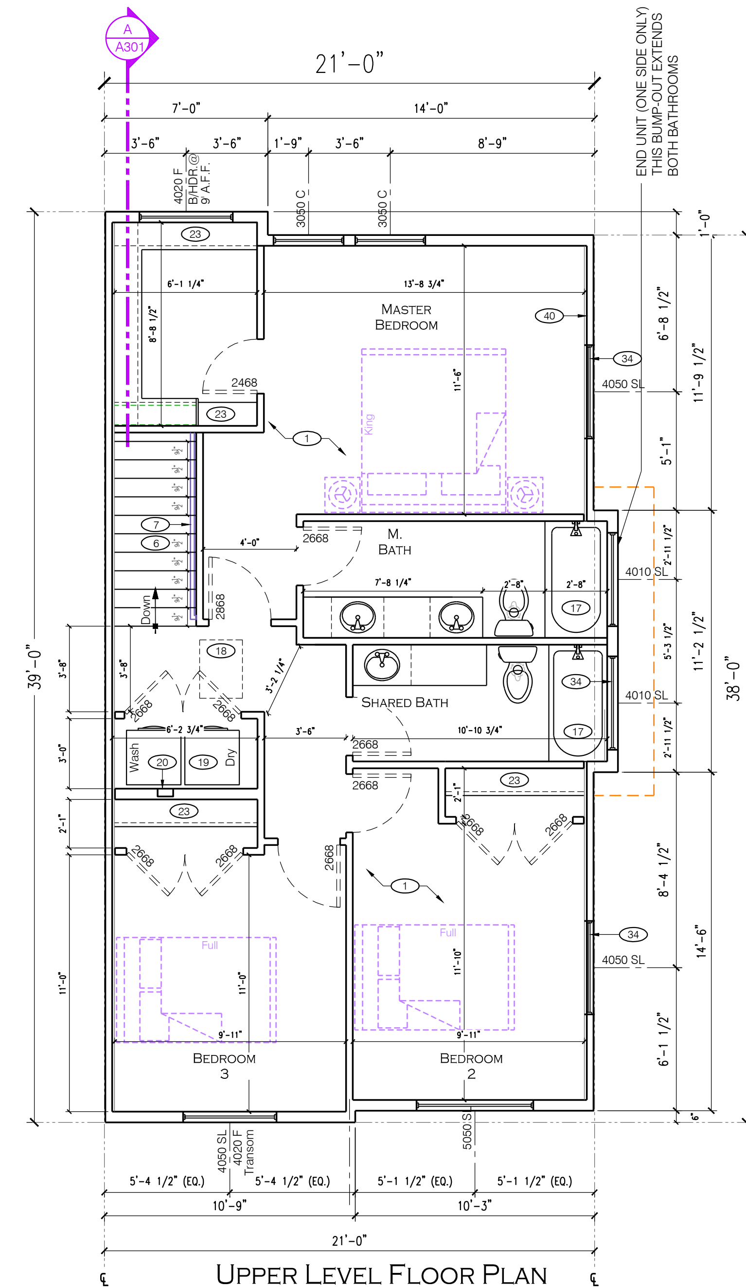
UPPER LEVEL FLOOR PLAN
