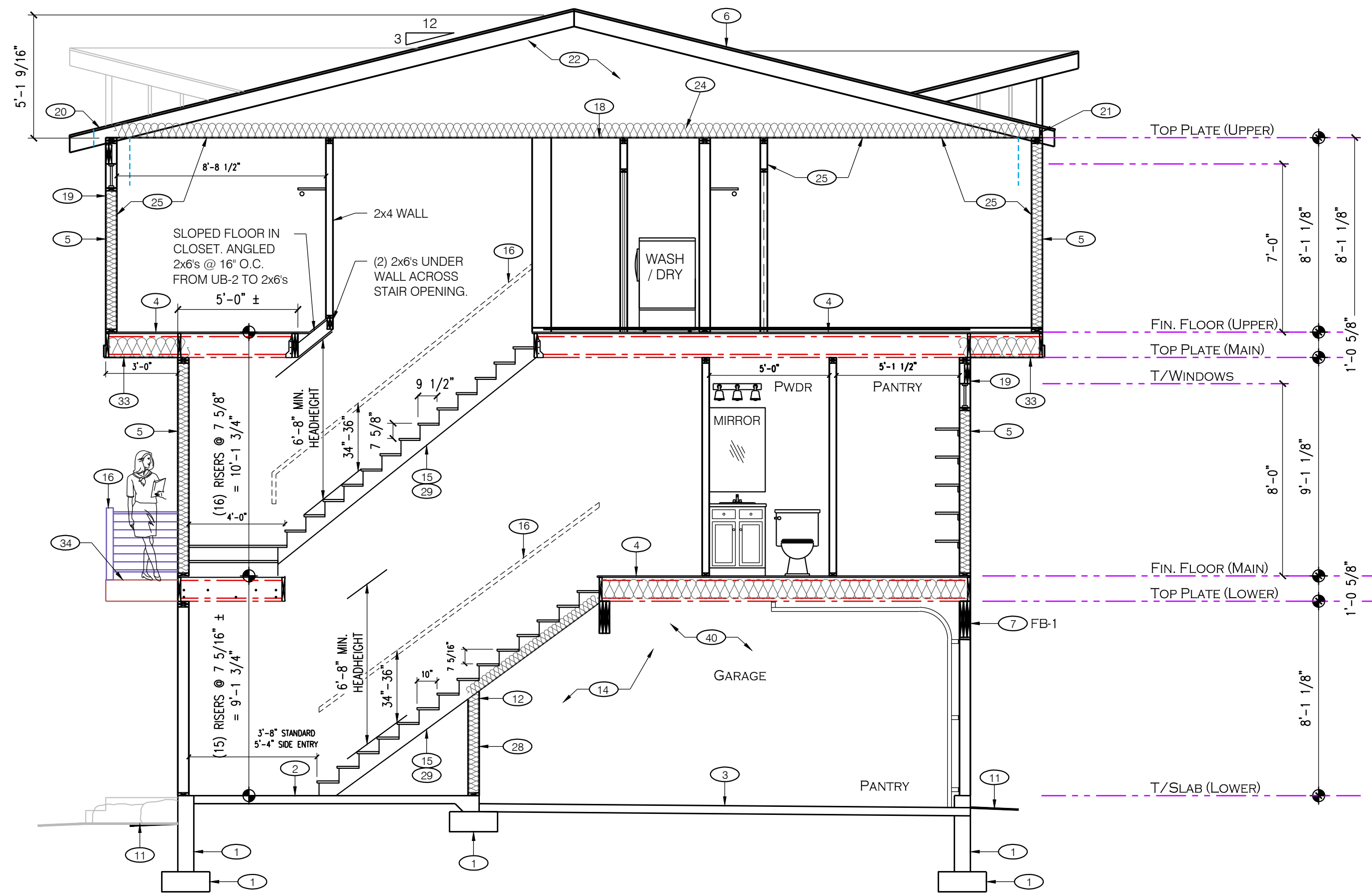
SECTION A
