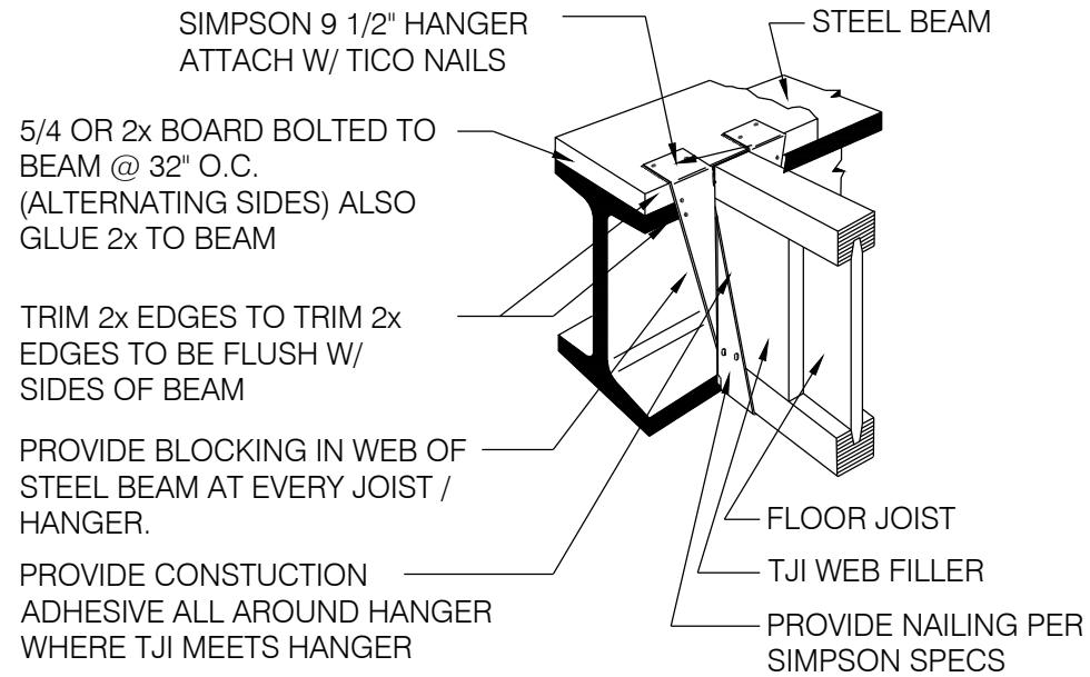
DETAIL OF STEEL BEAM OPTION W/ HANGERS
