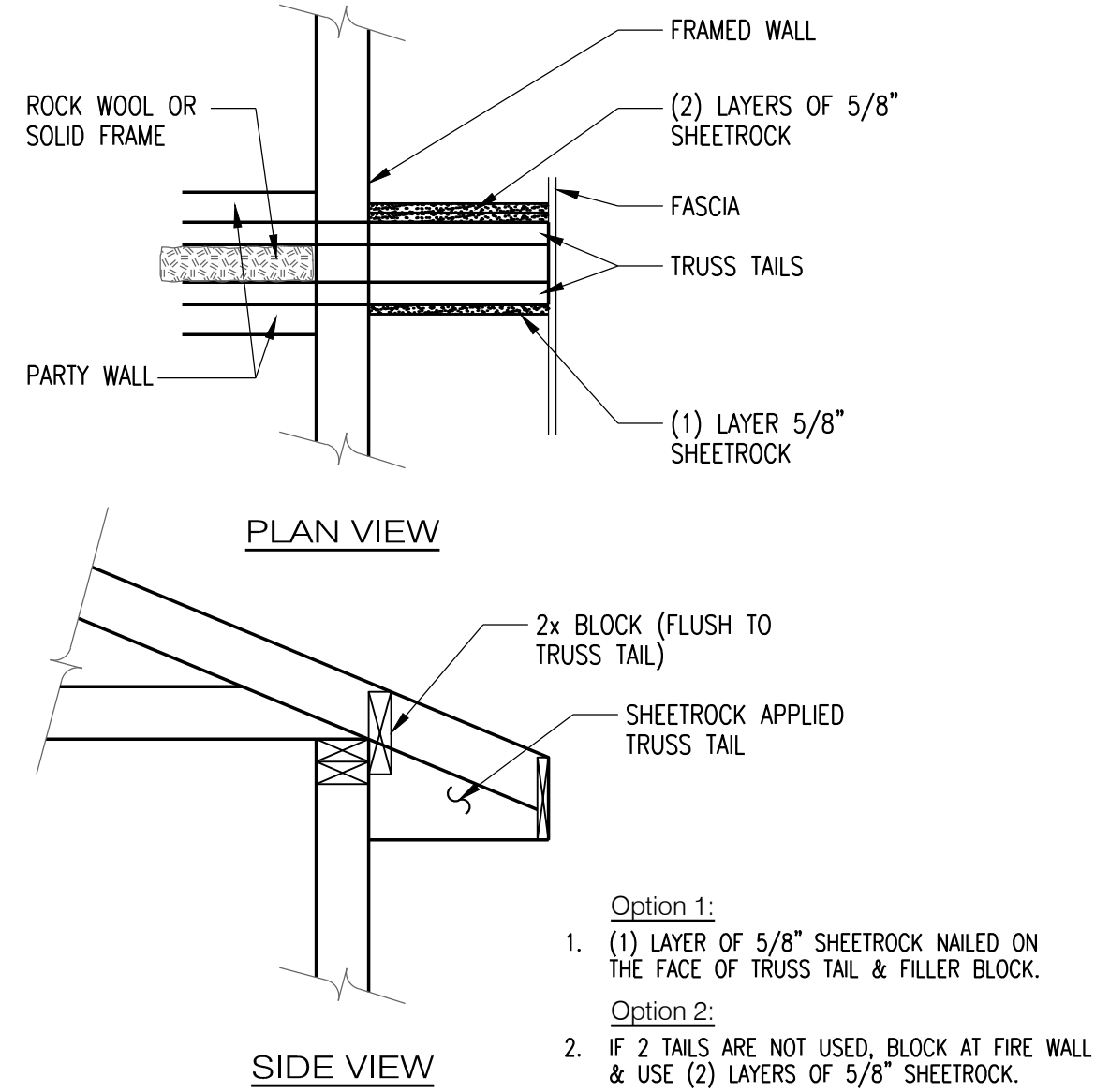
FIRE SEPARATION AT GABLE END TAILS 1/2" = 1'-0"
