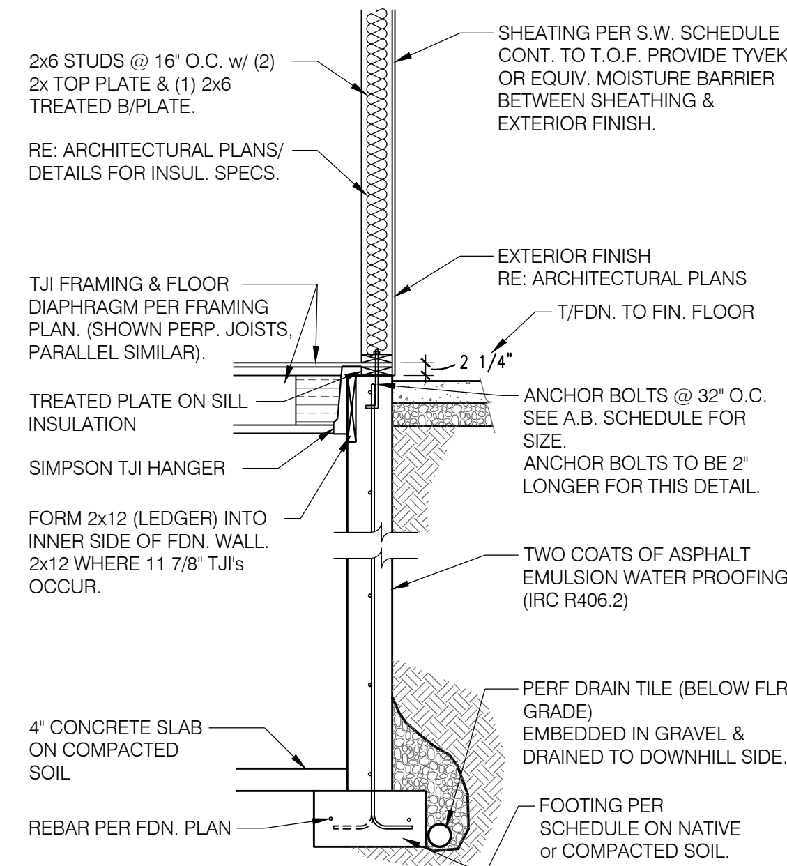
6 TYPICAL WALL SECTION AT FULL HEIGHT FDN. WALL. 2x SCALE LISTED IN TITLEBLOCK
