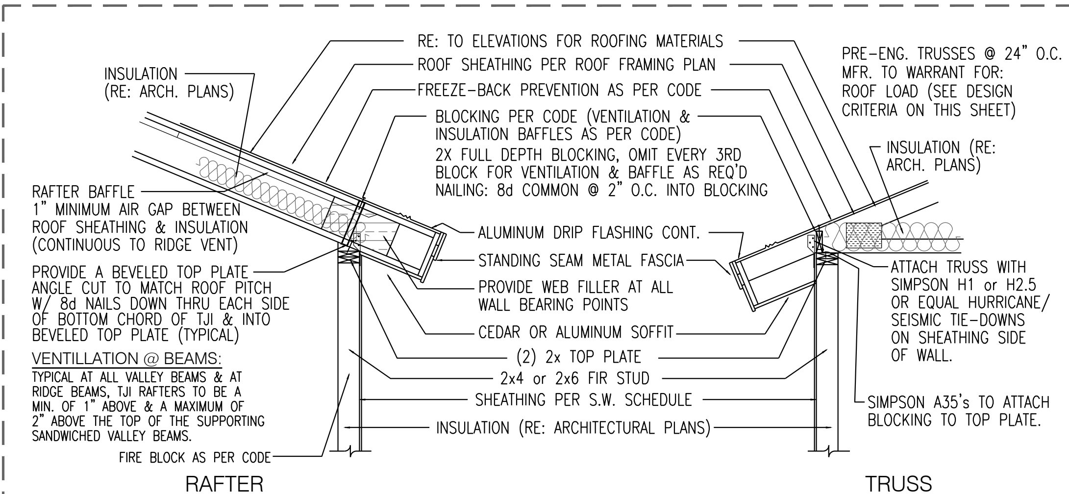
7 ROOF / SOFFIT / FASCIA / BLOCKING DETAIL 2x SCALE LISTED IN TITLEBLOCK
