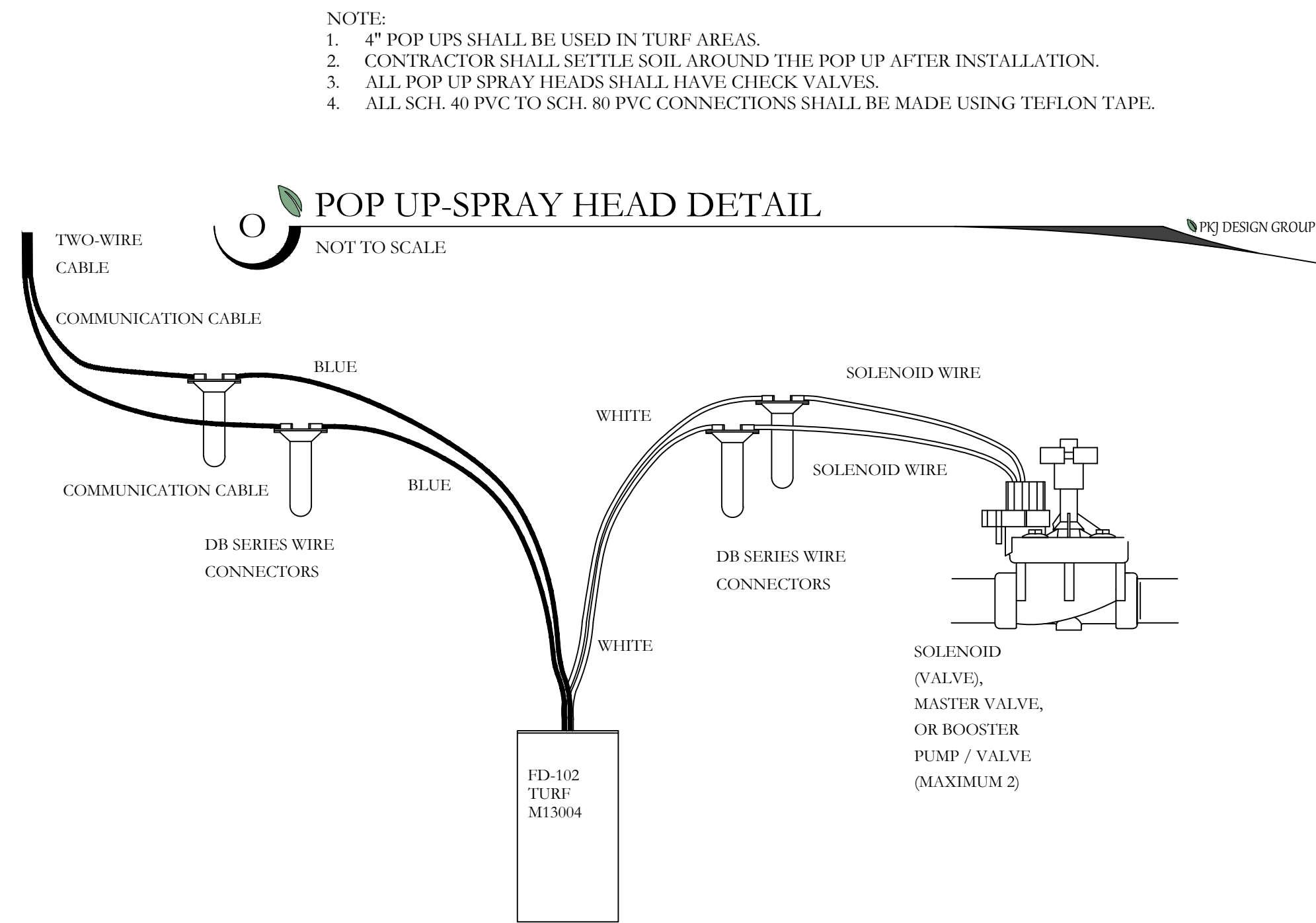
O POP UP-SPRAY HEAD DETAIL NOT TO SCALE
