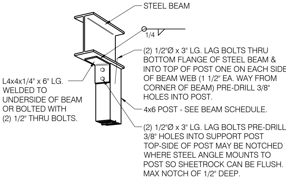
CONNECTION DETAIL
