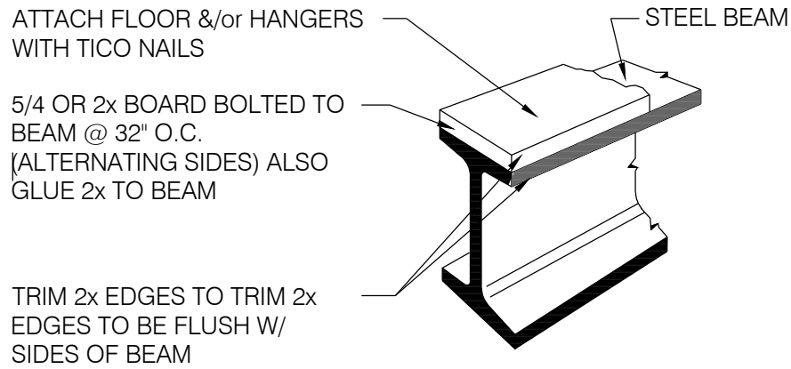
DETAIL OF STEEL BEAM
