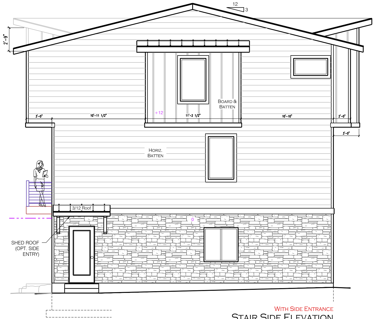
With Side Entrance STAIR SIDE ELEVATION
