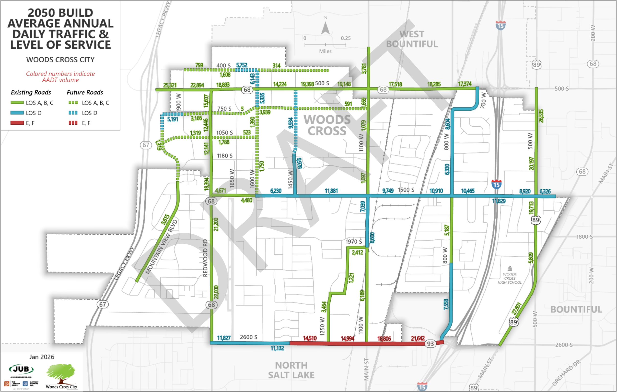
Figure 9: 2050 AADT/LOS
