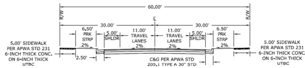
2 SINGLE FAMILY RESIDENTIAL PRIVATE STREET SCALE: 1" = 10'
