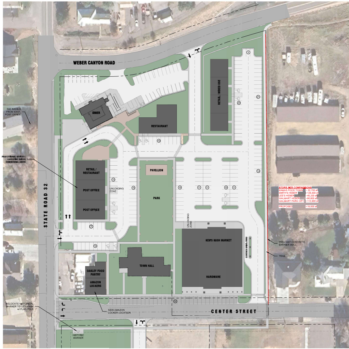
1 SITE PLAN - MASTER PLAN COLOR - NORTH SHEET 1 - 01V
