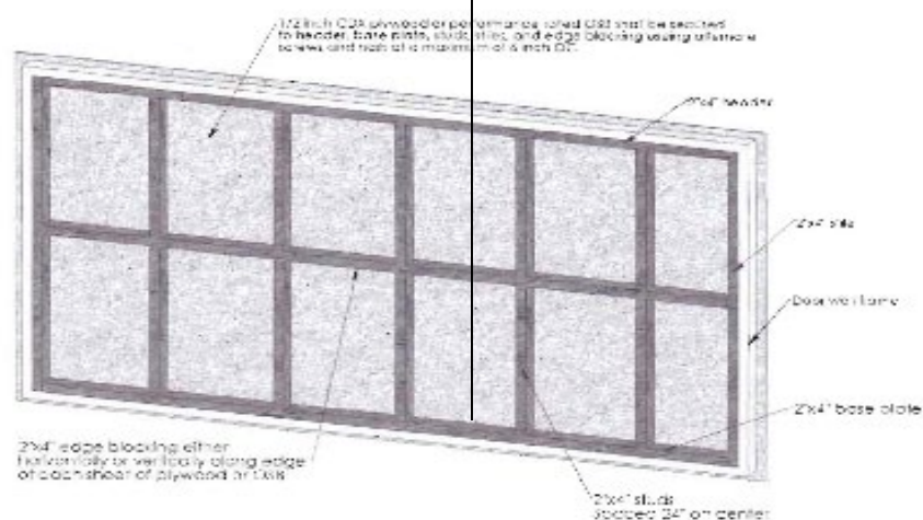
FIGURE A102.1(2) BOARDING OF DOOR WALL
