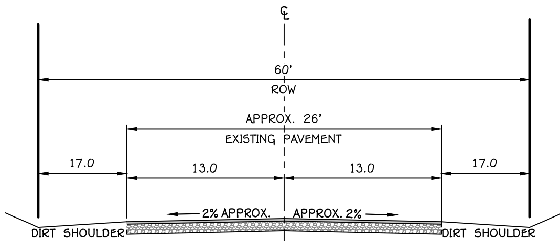
SILVER REEF ROAD CROSS SECTION
