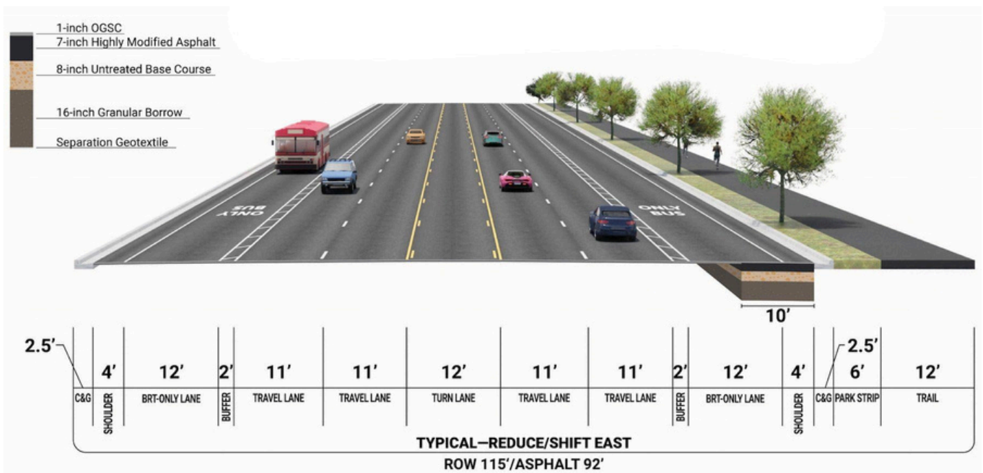
Figure 1 - Dedicated Transit Lanes on SR-224 from Kimball Junction to Kearns Boulevard
