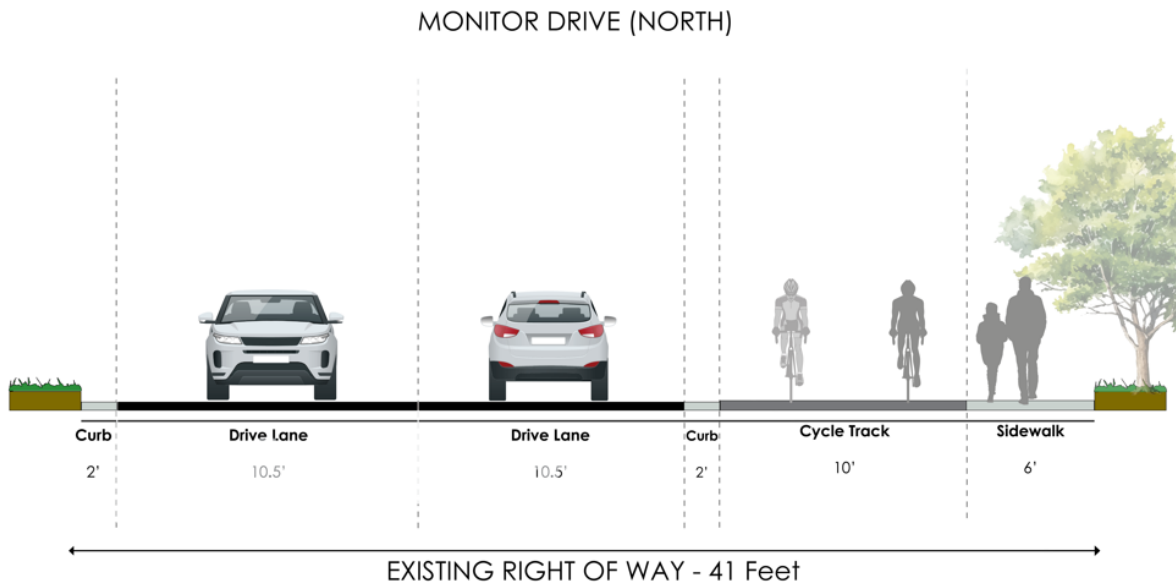
Figure 1 Shows typical cross sections planned for Monitor Drive north of Kearns Boulevard and south of Little Kate Road.
