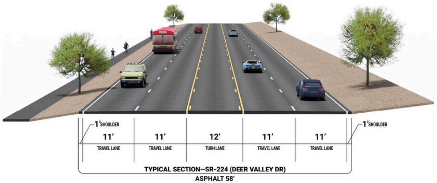
Figure 3 - Mixed Flow Lanes on Deer Valley Drive from SR-224 to Old Town Transit Center
