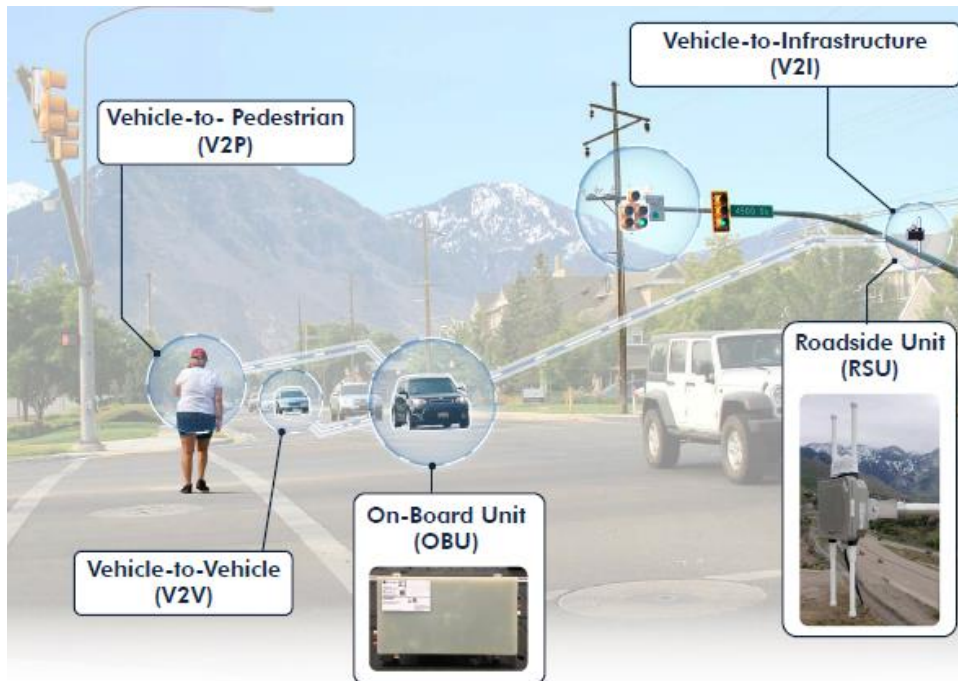
Figure 1 Illustration of the Connected Vehicle Communication Ecosystem –showing the various Vehicle-to-Everything (V2X) communication types, including Vehicle-to-Pedestrian (V2P), Vehicle-to-Vehicle (V2V), and Vehicle-to-Infrastructure (V2I), enabled by On-Board Units (OBU) in vehicles and Roadside Units (RSU) integrated with traffic infrastructure.
