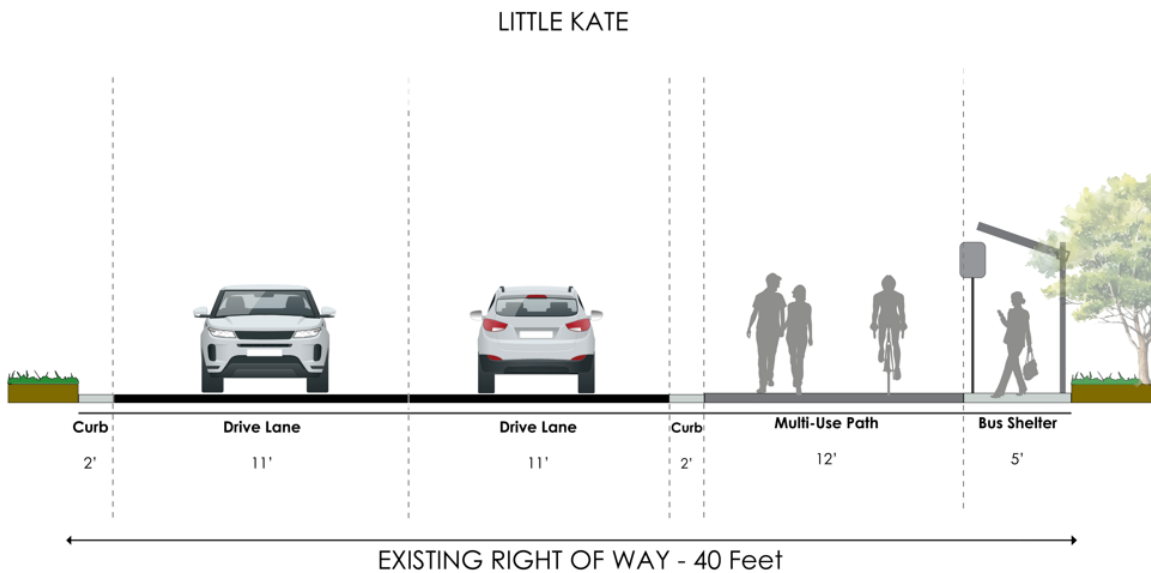
Figure 2 Shows cross sections planned for Little Kate Road between Lucky John Drive and Holiday Ranch Loop Road.
