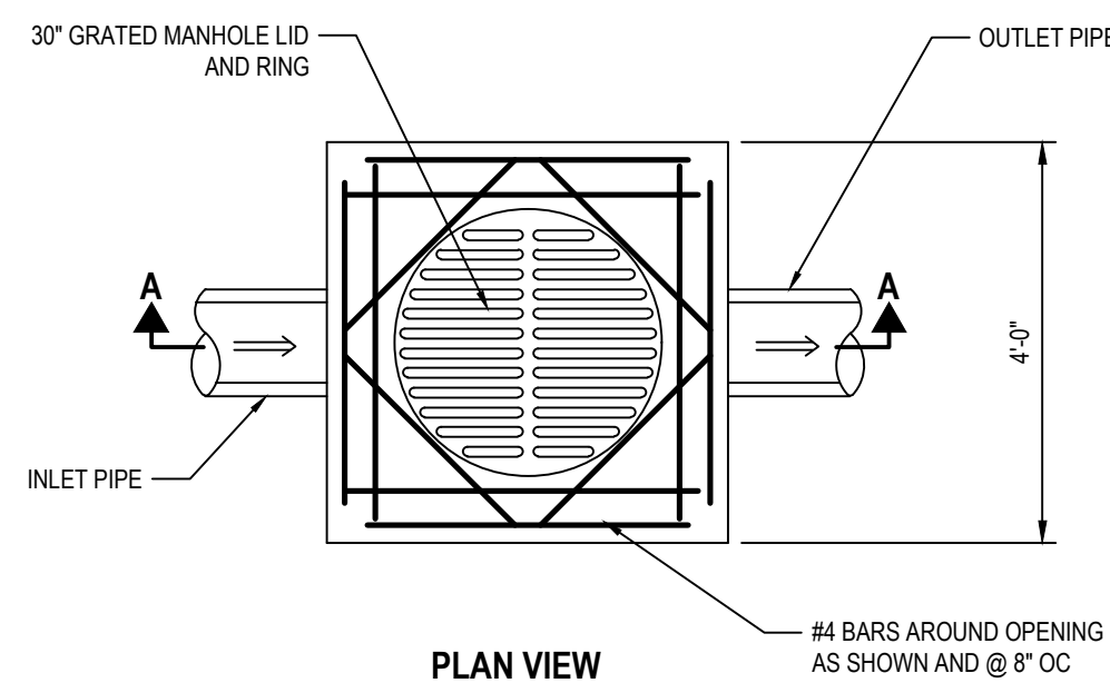
PLAN VIEW
