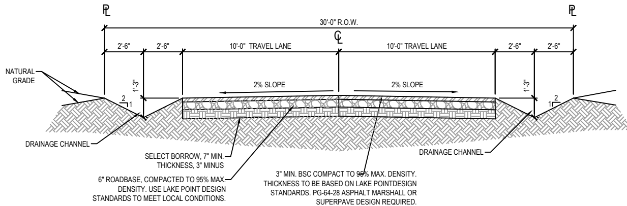
2 30'-0" ROW PRIVATE ROAD CROSS SECTION
