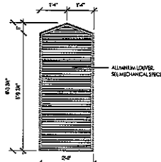
ALUMINUM LOUVER DETAIL 1/2" = 1'-0"
