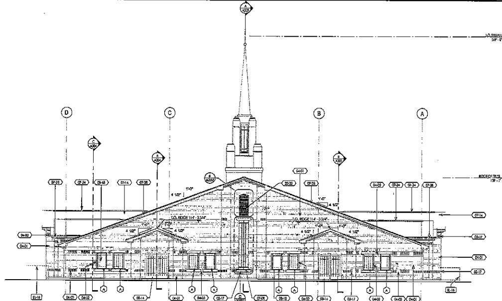
REAR ELEVATION 1/8" = 1'-0"
