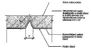
EIFS - SECTION 1" = 1'-0"
