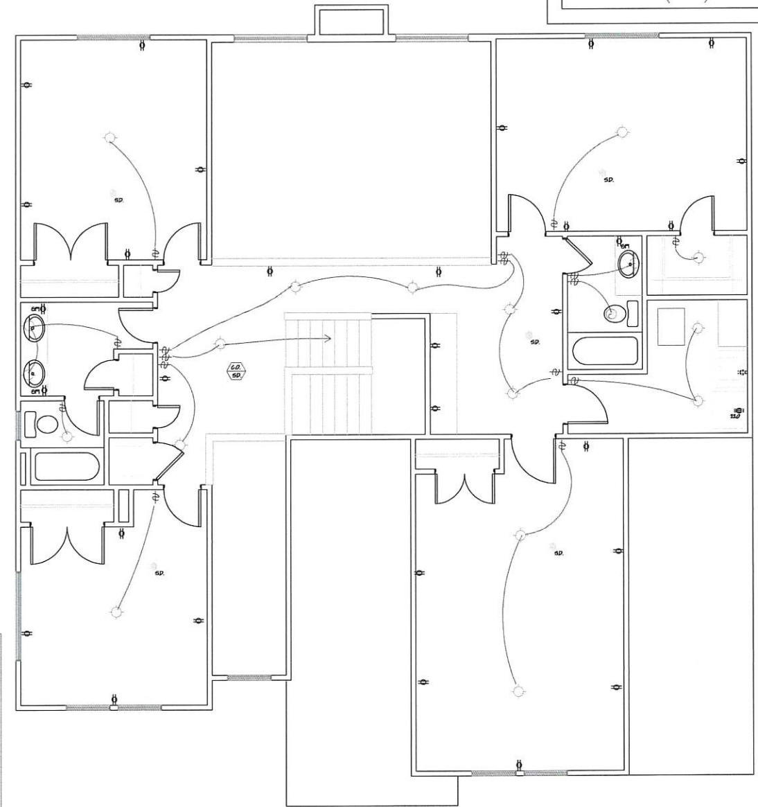
ELECTRICAL PLAN UPPER FLOOR
