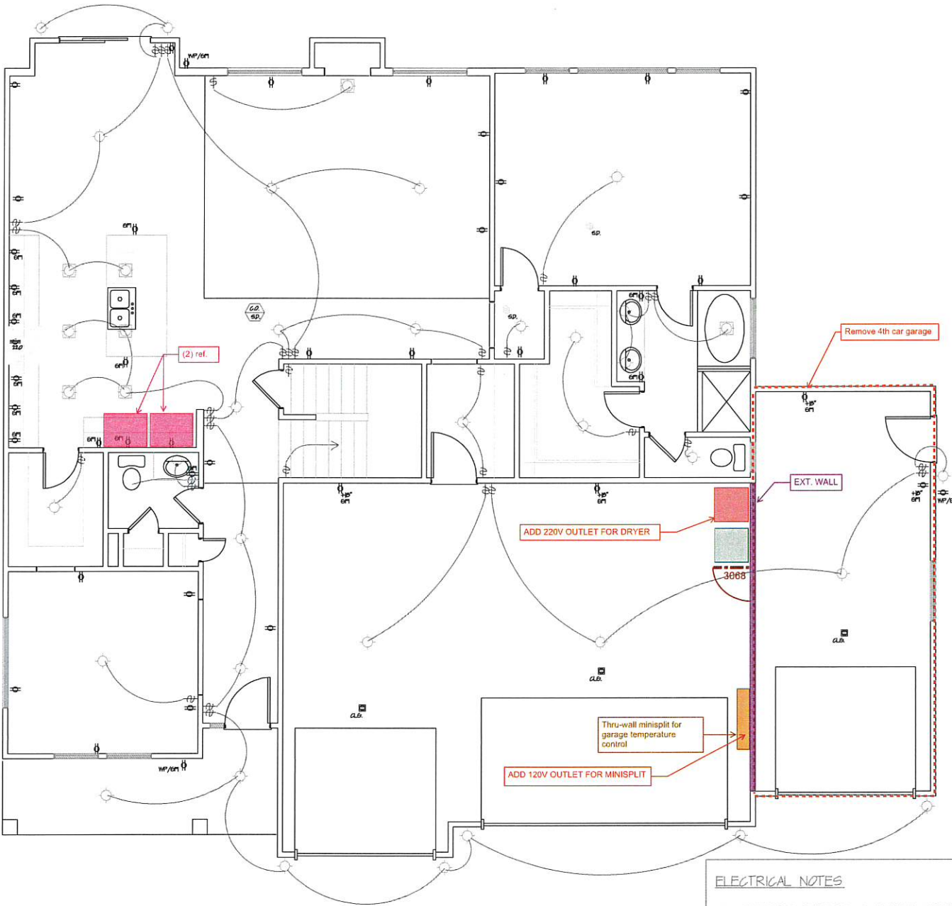
ELECTRICAL PLAN MAIN FLOOR
