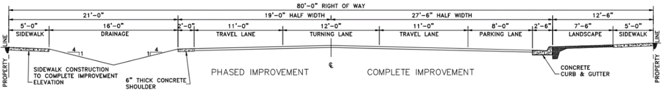
80' CONDITIONAL COLLECTOR ROADWAY SECTION A
