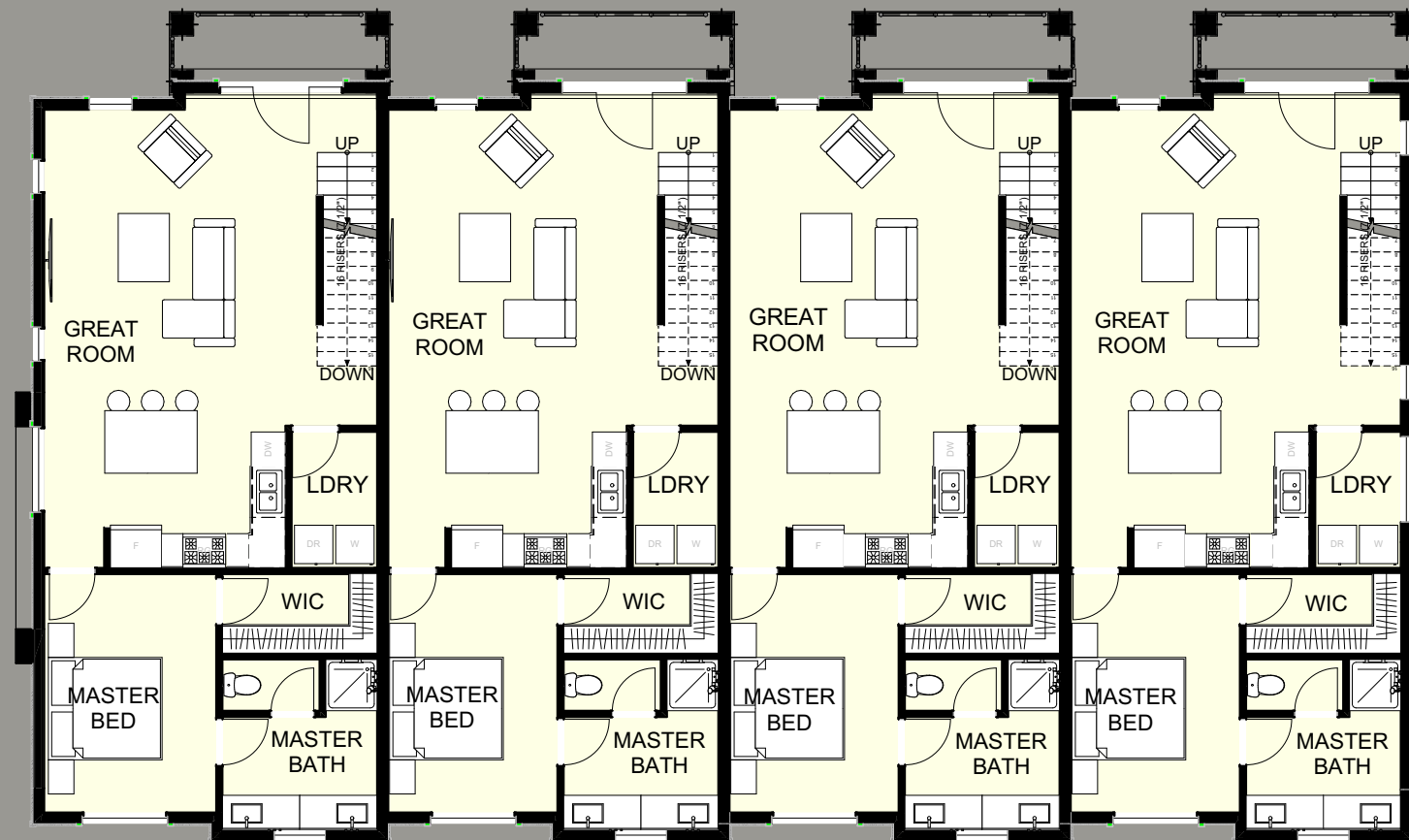
3-Story Options - 2ND FLOOR PLAN
